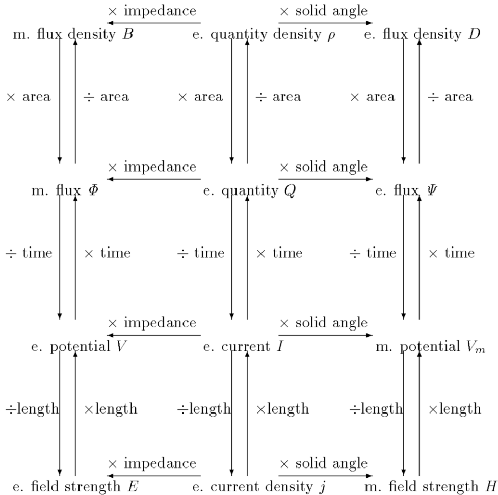
Figure 1. Symmetric arrangement of electromagnetic quantities.
