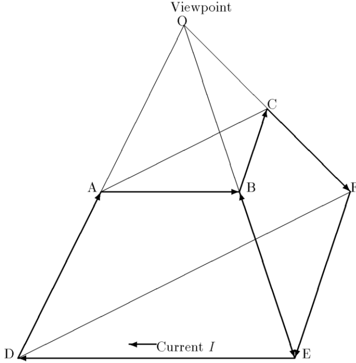
Figure 2. Magnetic scalar potential as current \times subtended solid angle.
