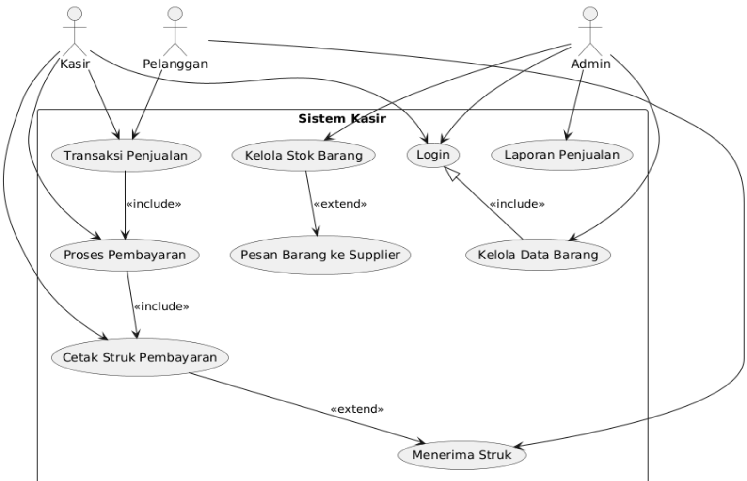
Use Case Diagram - Sistem Kasir
