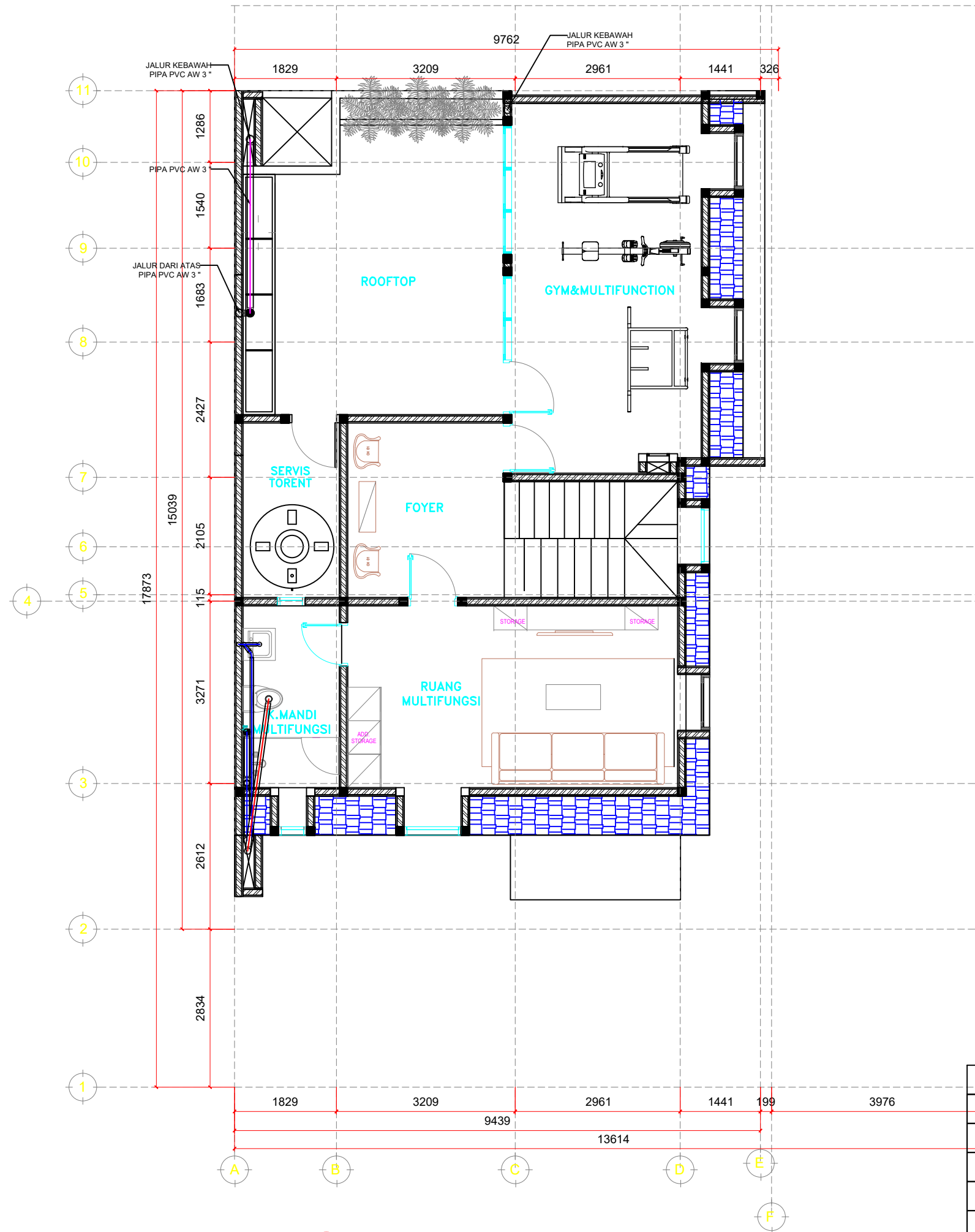
01 DENAH AIR KOTOR,AIR BEKAS,AIR HUJAN LT.4 1 : 100
