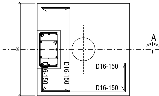
FOUNDATION DETAILS TYPE F2 SCALE 1:25
