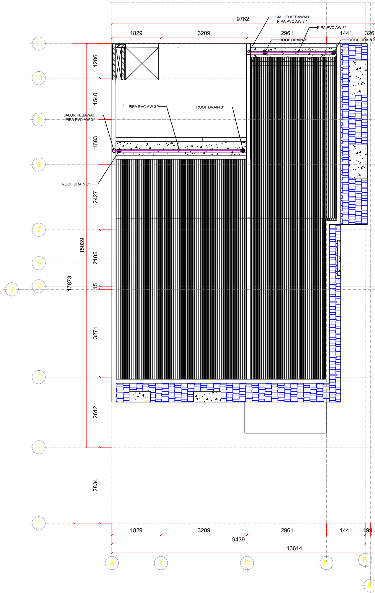
01 DENAH AIR KOTOR,AIR BEKAS,AIR HUJAN ATAP
