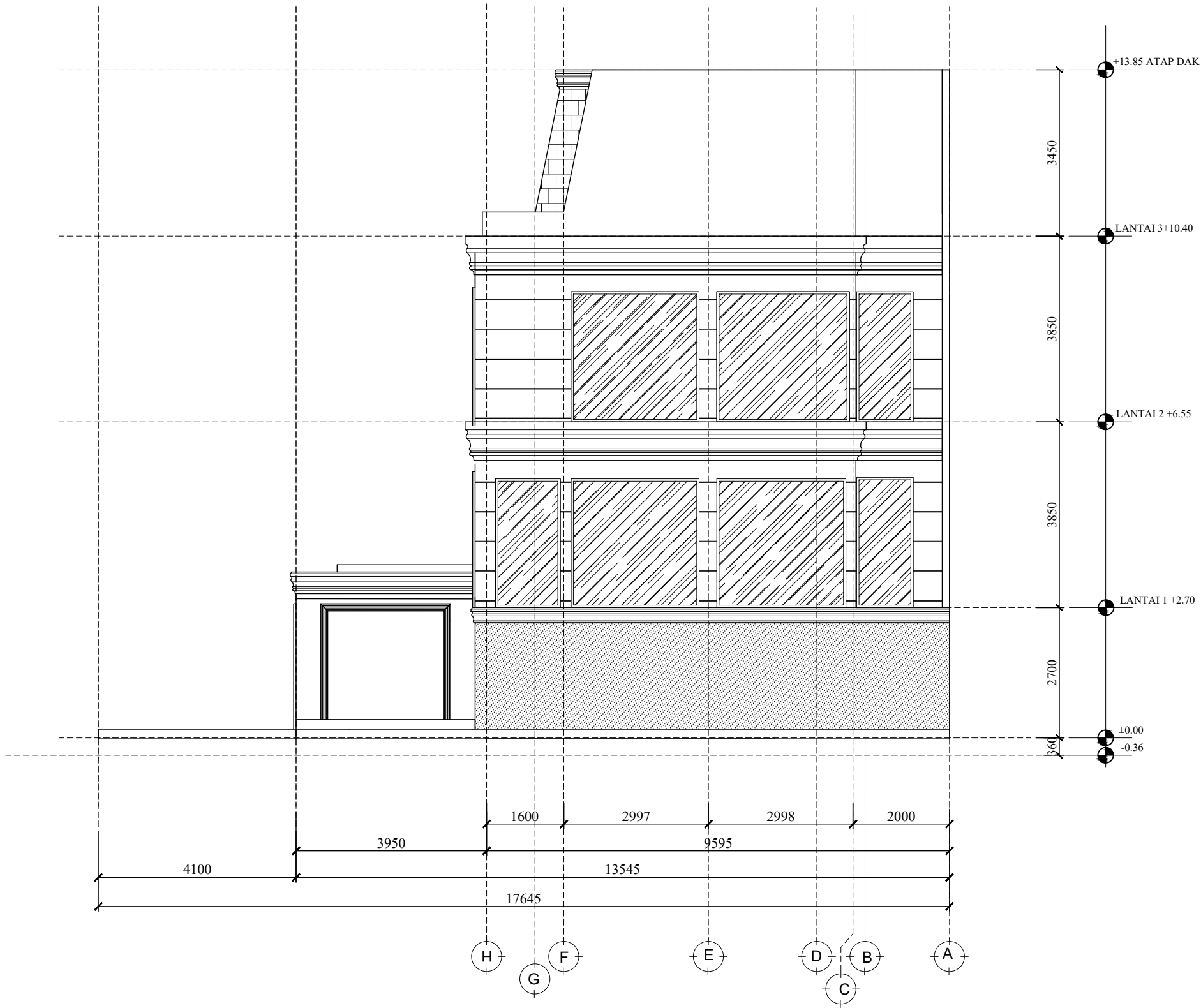
01 REAR ELEVATION 1 : 100
