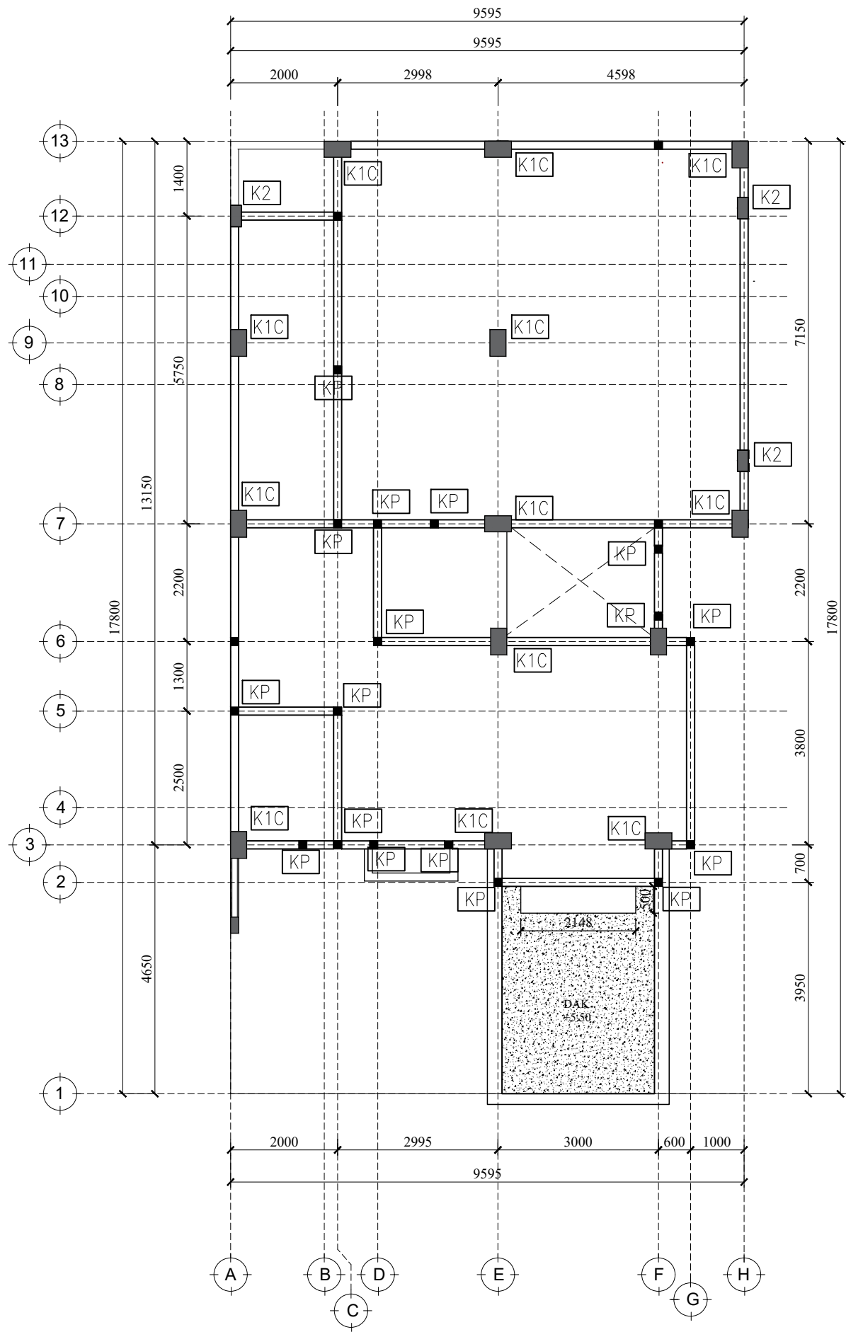
01 2ND COLUMN FLOOR PLAN 1 : 100
