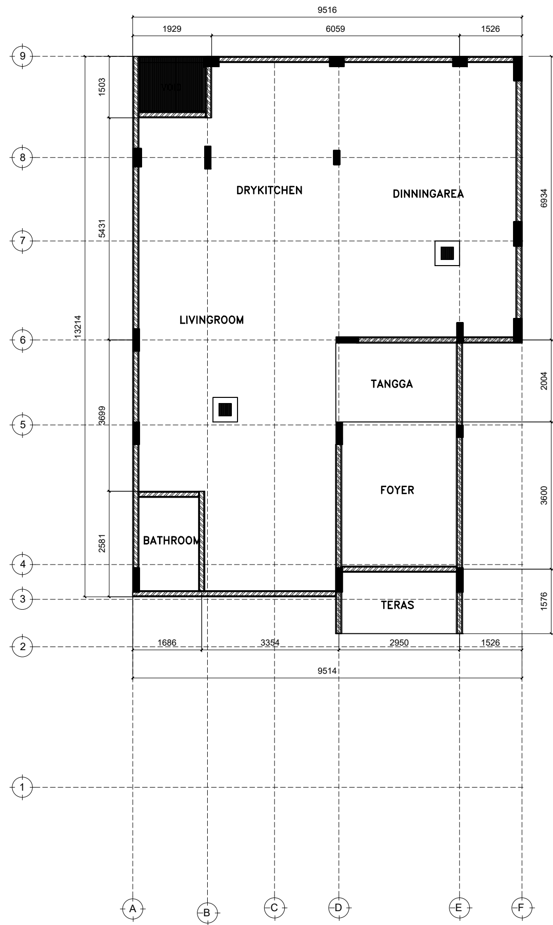
01 1ST FLOOR PLAN 1:100
