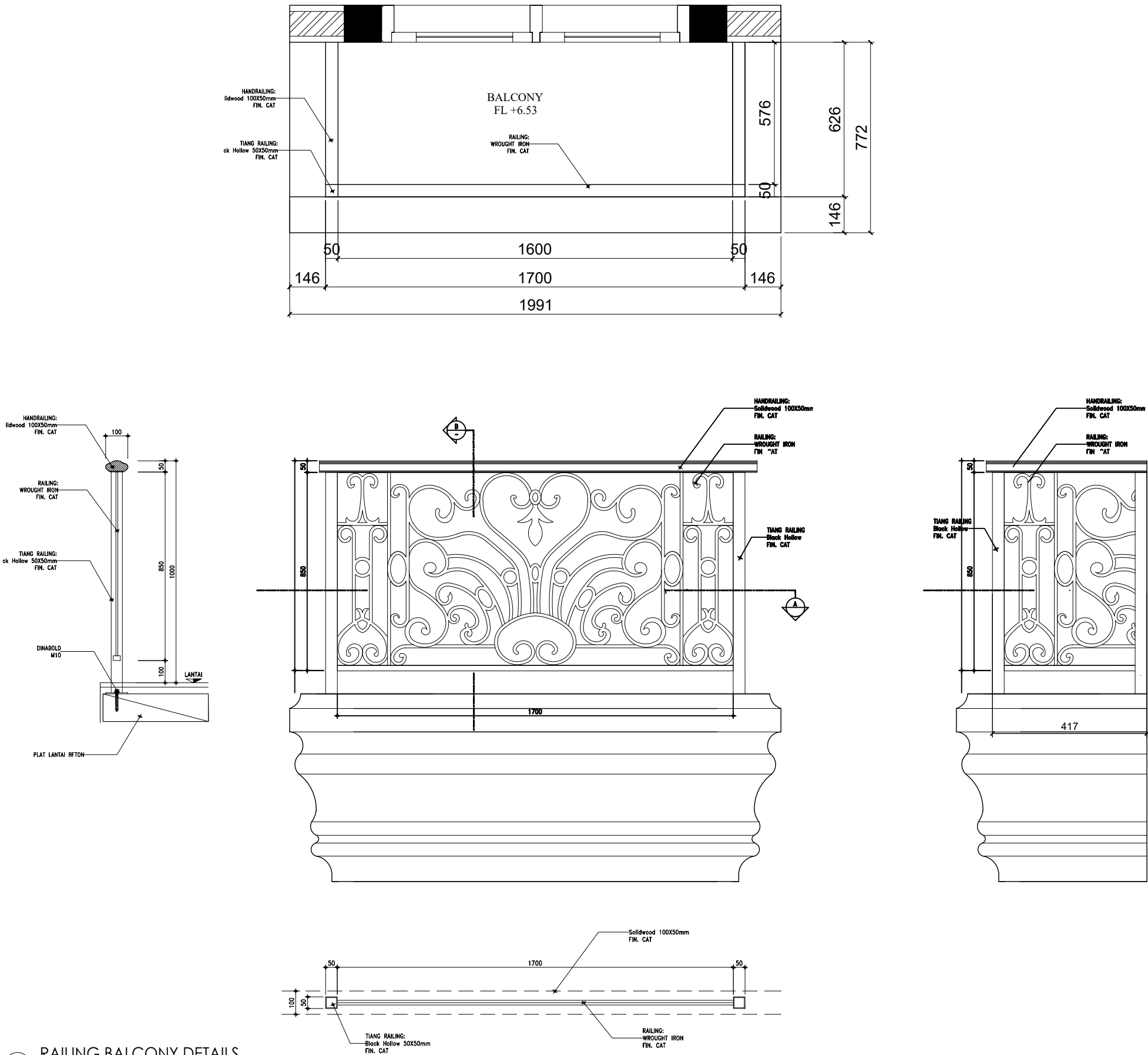
RAILING BALCONY DETAILS SCALE 1:15
