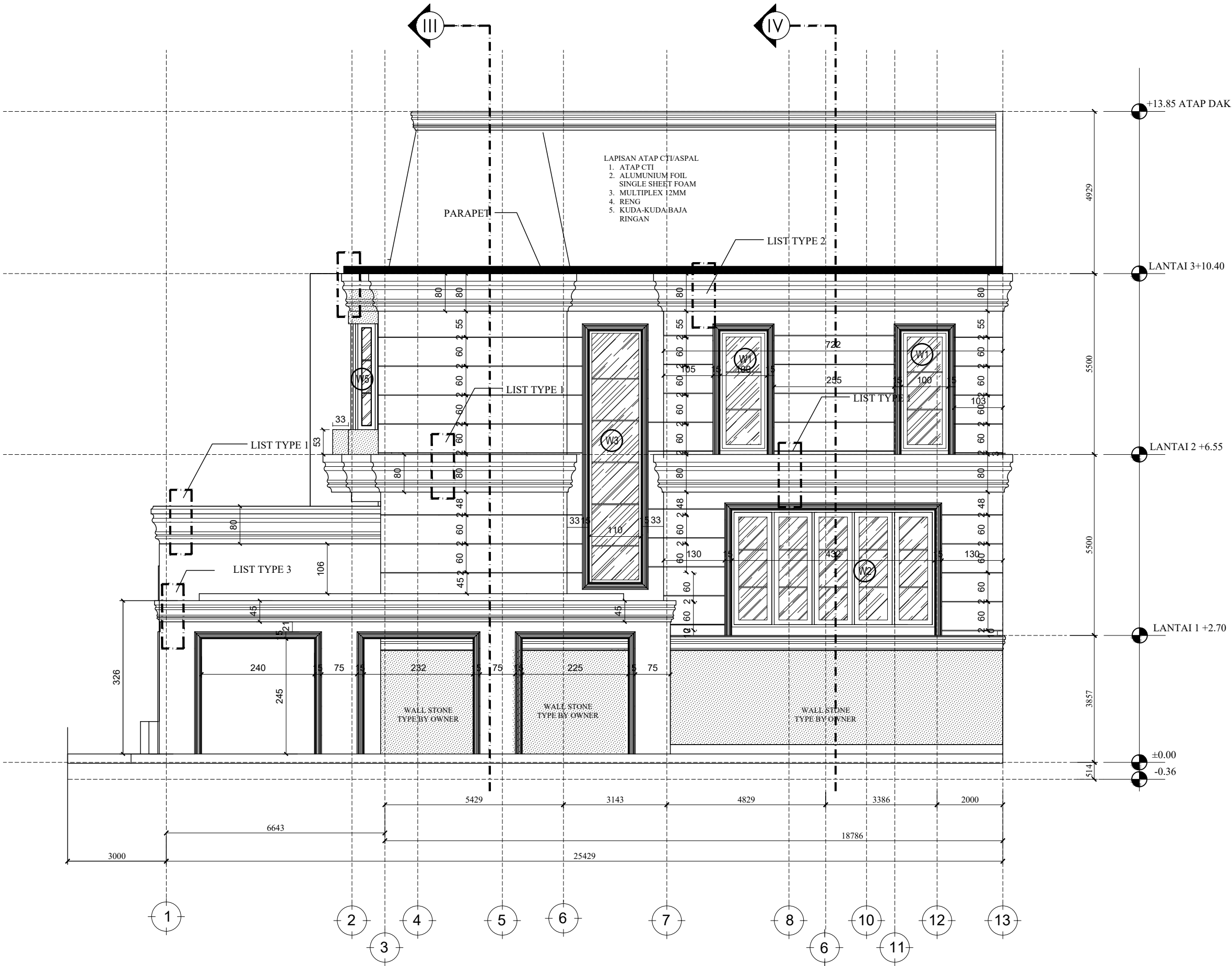
RIGHT ELEVATION DETAIL FASAD SCALE 1:70
