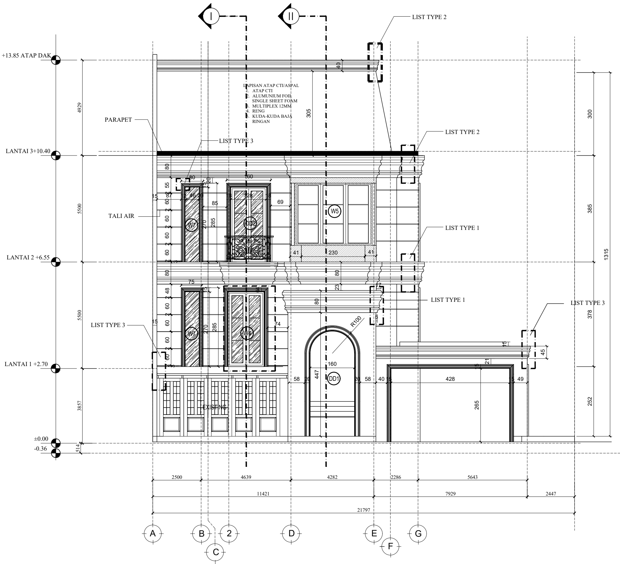
FRONT ELEVATION DETAIL FASAD SCALE 1:70
