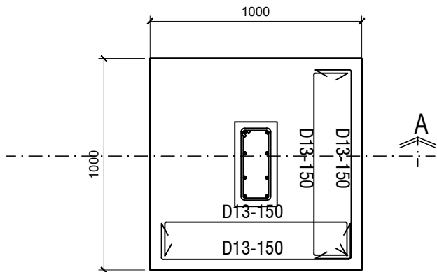
FOUNDATION DETAILS TYPE F3 SCALE 1:25
