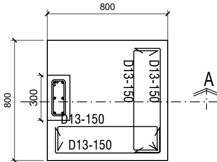
FOUNDATION DETAILS TYPE F4 SCALE 1:25
