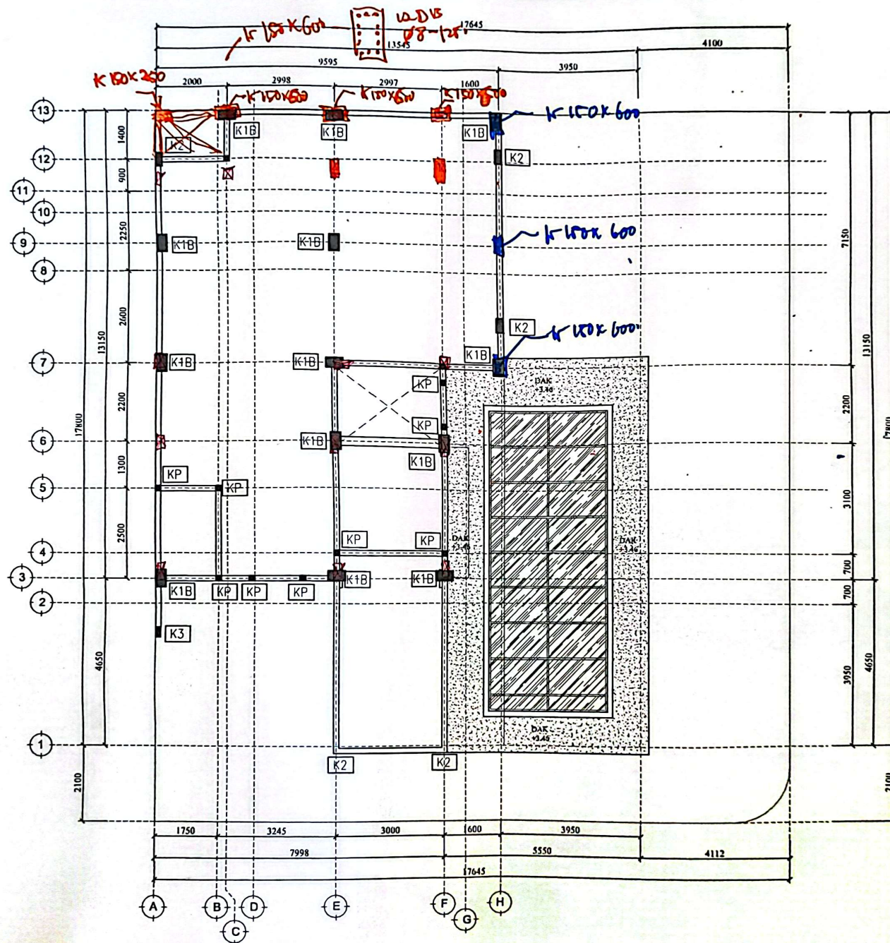
01 1ST COLUMN FLOOR PLAN 1:100
