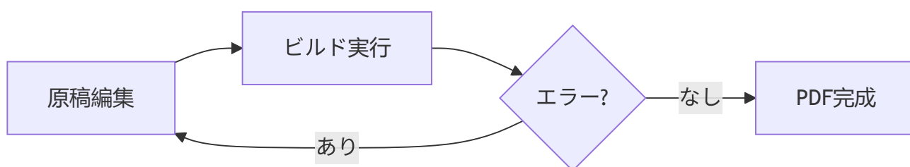
Mermaid diagram
