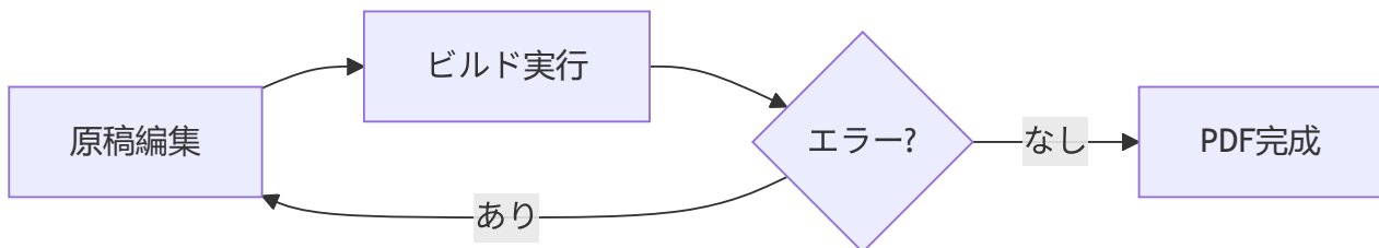
Mermaid diagram
