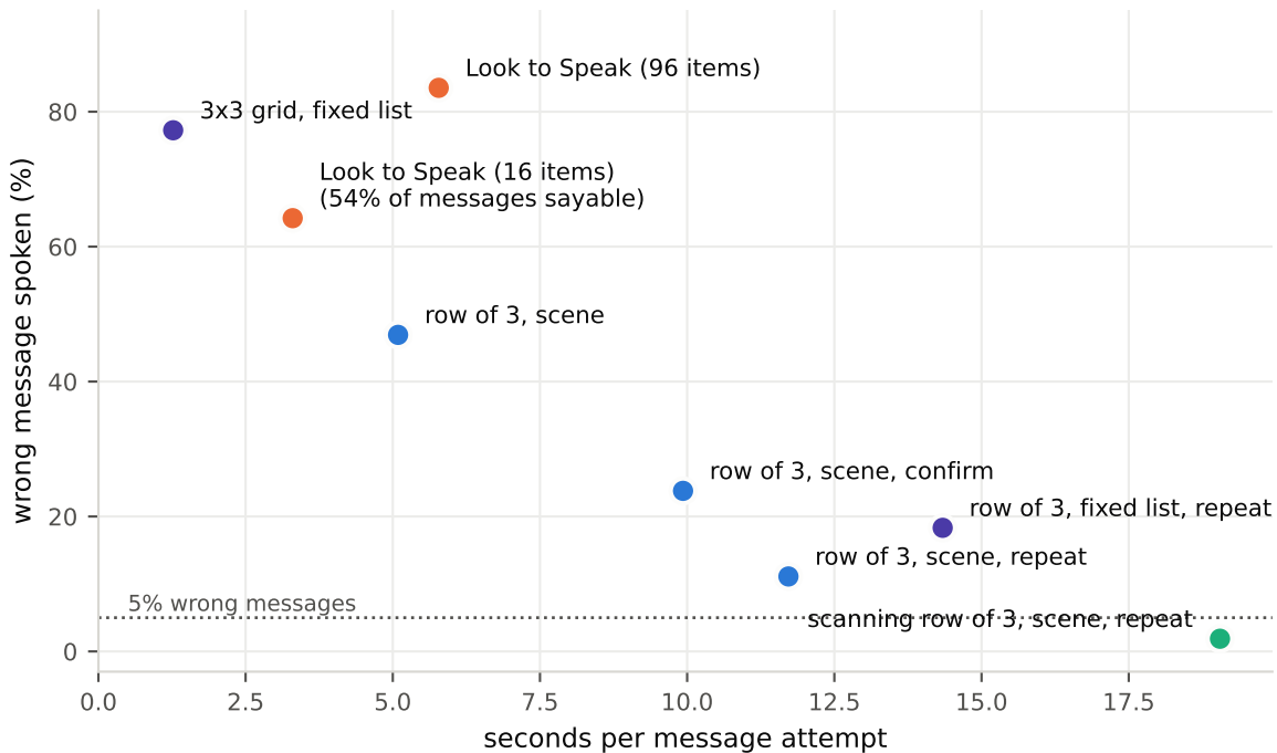
Speed against error, at the gaze accuracy measured in Study 1
