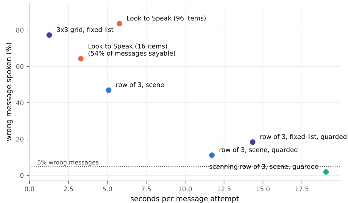
Speed against error, at the gaze accuracy measured in E1b
