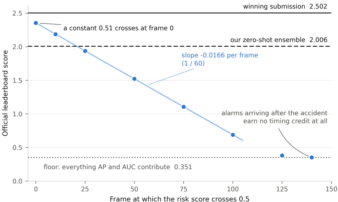
Figure 2: The official score is a straight line in the frame at which the alarm fires. Points are video-blind submissions scored by the organisers; the fit is over crossings up to frame 100. A constant crosses at frame 0.
