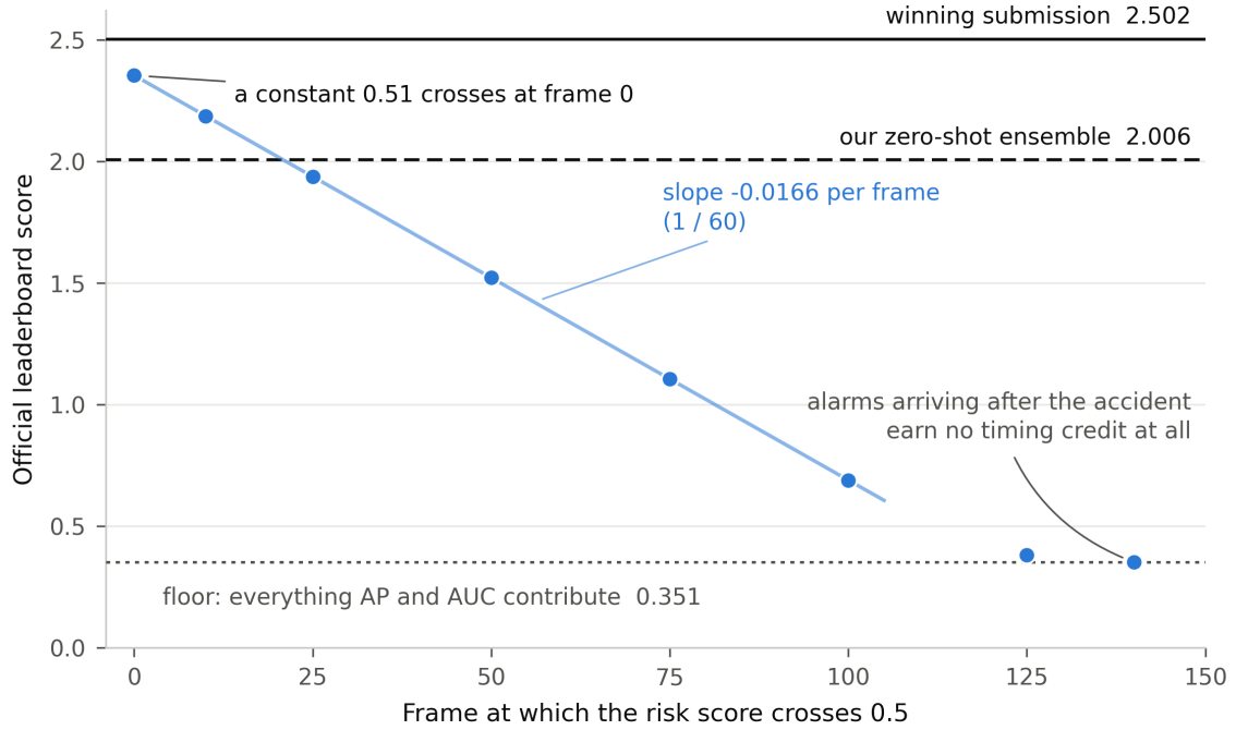
Figure 1: The official score is a straight line in the frame at which the alarm fires. Points are video-blind submissions scored by the organisers; the fit is over crossings up to frame 100. A constant crosses at frame 0.
