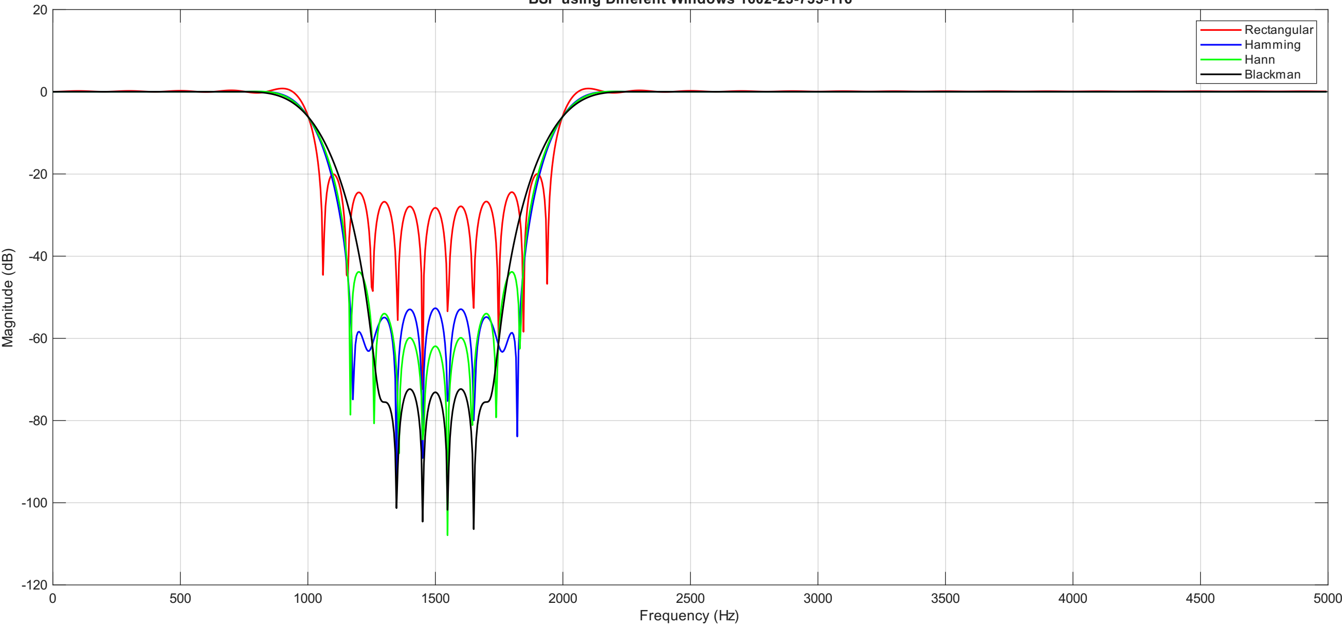
BSF using Different Windows 1602-23-735-116
