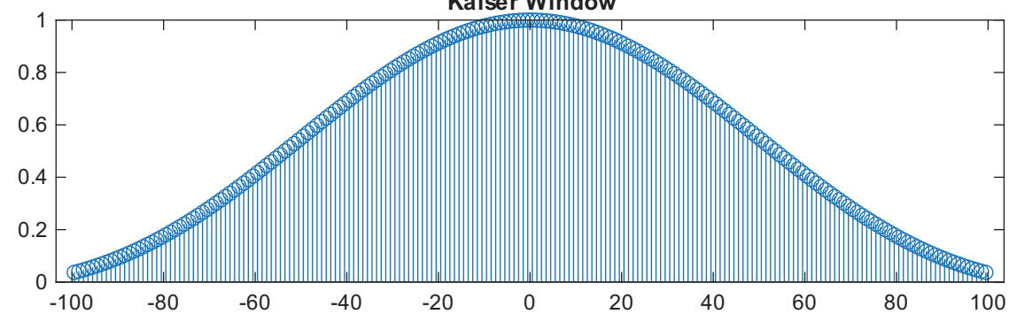
Kaiser Window
