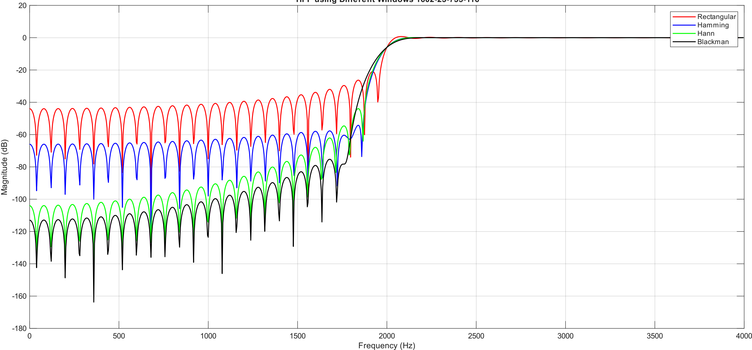
HPF using Different Windows 1602-23-735-116
