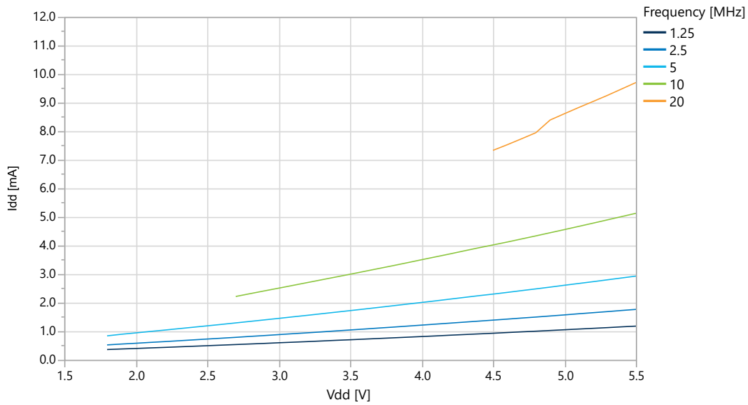
Figure 33-5. Active Supply Current vs. V_{DD} ( f = [1.25, 20] MHz) at T = 25^\circ\text{C}
