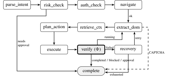
Fig. 2. Execution graph compiled in graph.py. Only the shaded verify node can end a task as COMPLETED, and only when \Phi holds. A CAPTCHA seen during observation ends it as BLOCKED. Not drawn: failures in parse_intent and navigate also route to recovery.
