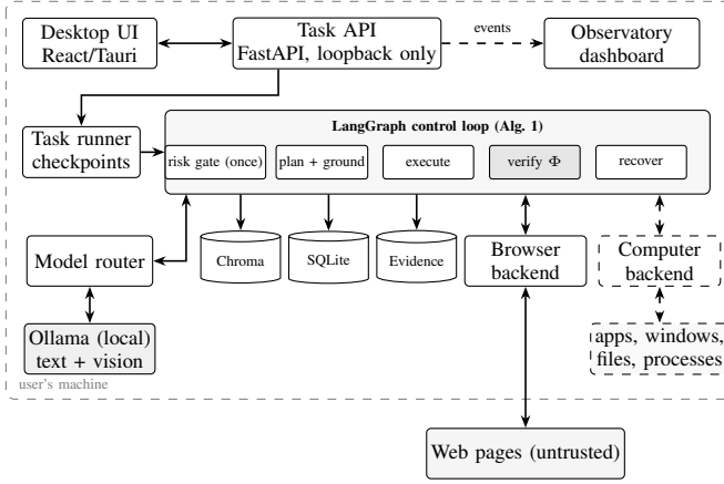
Fig. 1. Components of Agentic Pilot. Solid: implemented; dashed: proposed. Everything inside the boundary runs on the user’s machine; the model endpoint must be a loopback address unless the user overrides it. The browser backend is the only implemented execution environment; the computer backend and the local resources it would act on are a design (Appendix A). The Observatory also reads the task database and evidence files.
