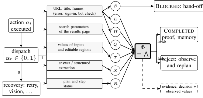
Fig. 2. Evidence-gated verification after an action (Algorithm 1, lines 7 and 22). A failed dispatch goes to recovery and never to \Phi . A successful dispatch makes the observed values available to the conjuncts of the browser predicate, each triggered by the wording of the goal (Section III); the bot-check condition \beta is tested first and hands the task to the user. Every decision is stored with the values it used.
