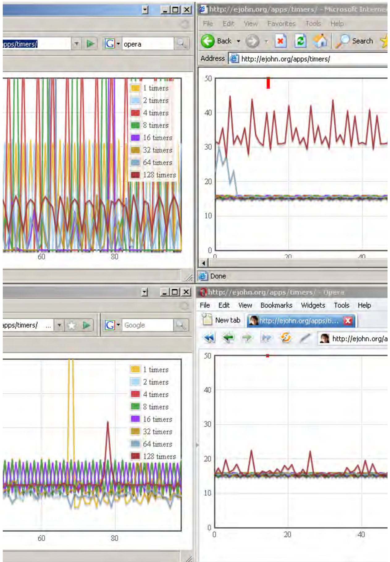
Windows Timers
