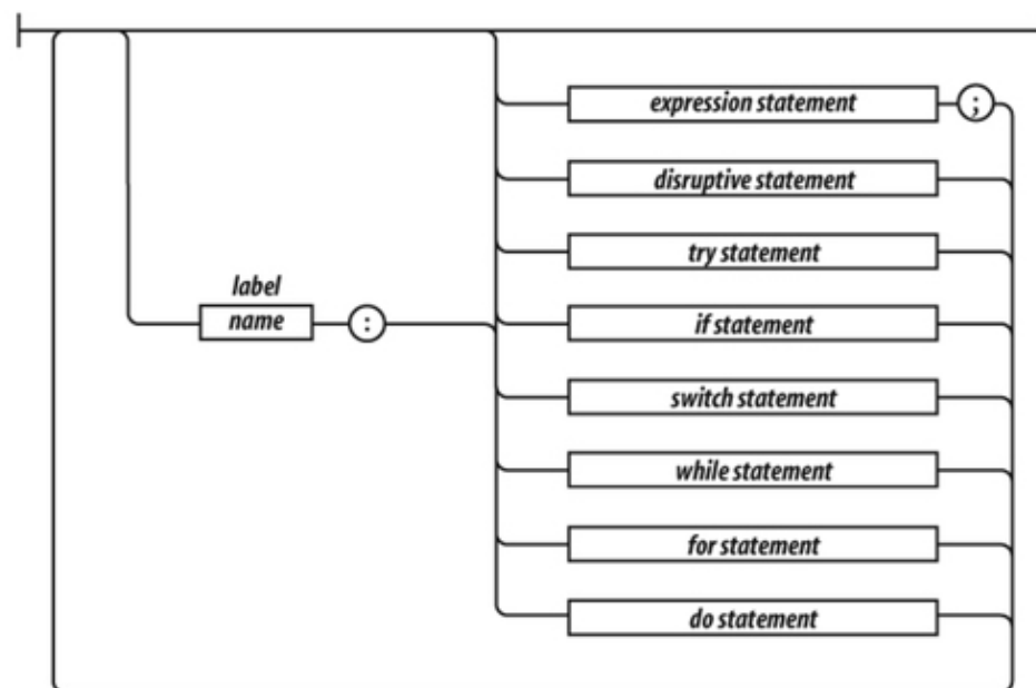
statements
