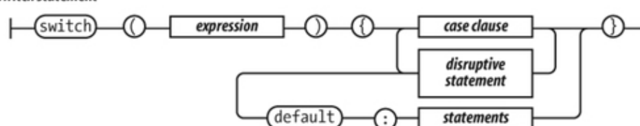
switch statement
