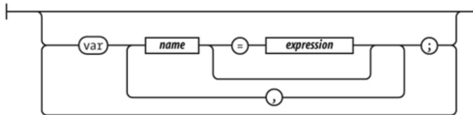
var statements
