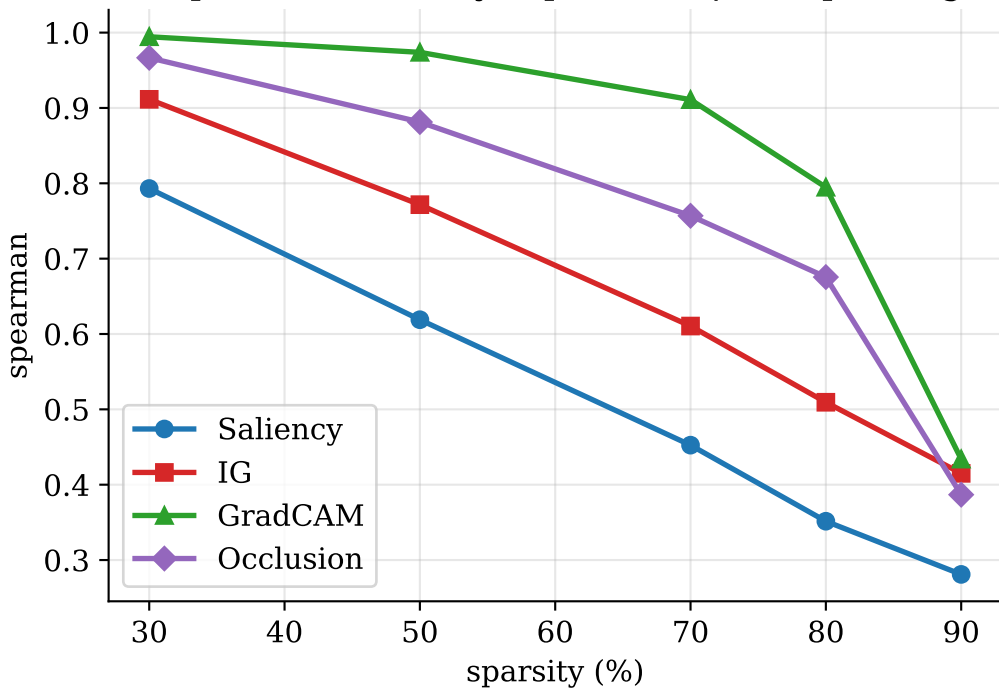
Explanation fidelity (Spearman \rho ) vs. pruning
