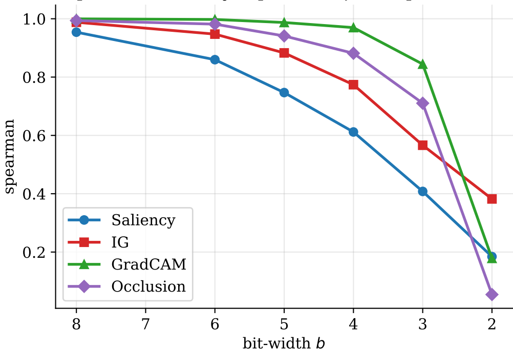
Explanation fidelity (Spearman \rho ) vs. quantization
