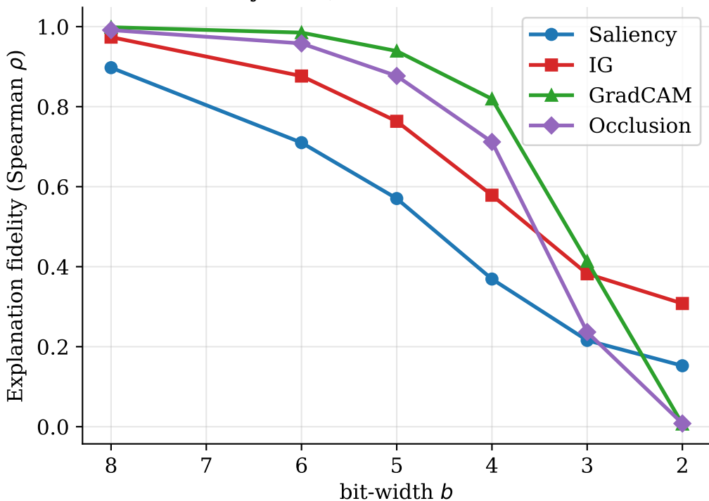
Fidelity vs. Quantization (CIFAR-10)
