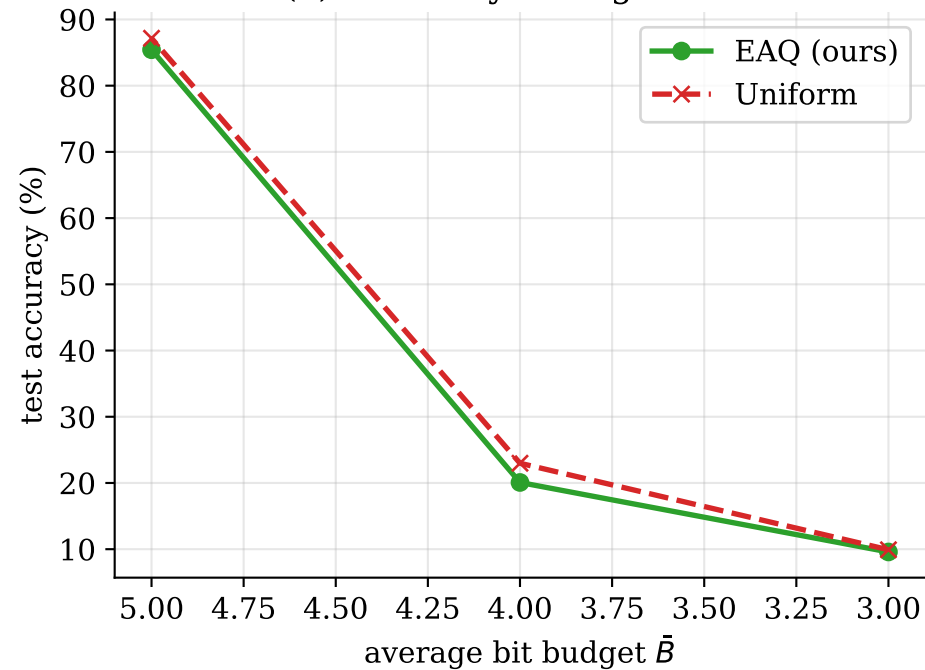
(a) Accuracy - ImageNette
