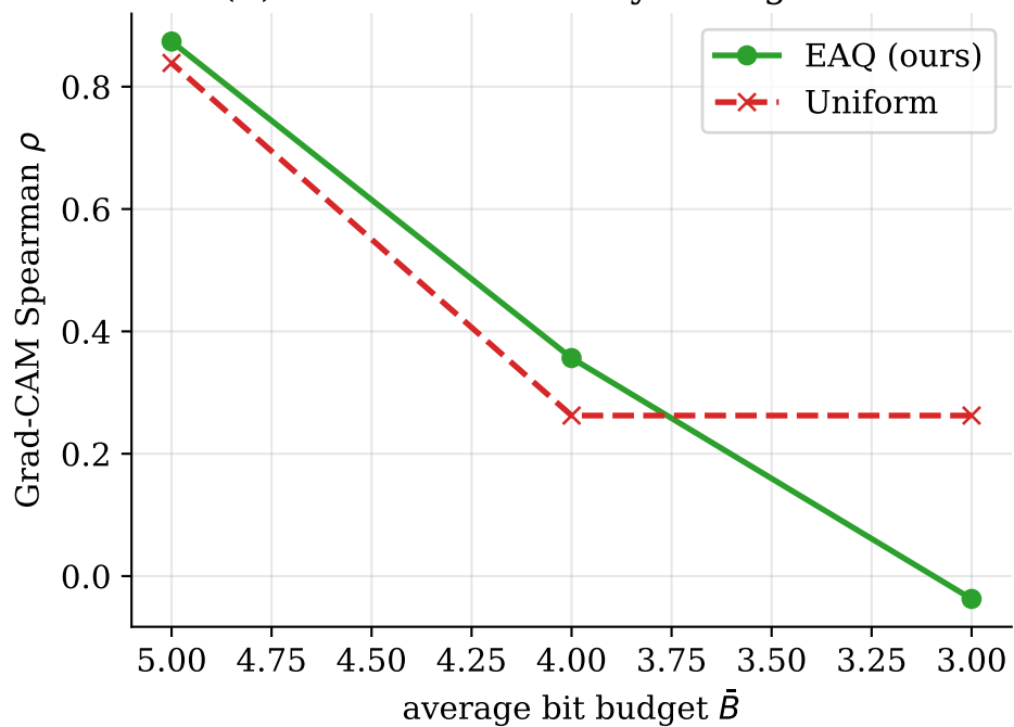
(b) Grad-CAM Fidelity - ImageNette
