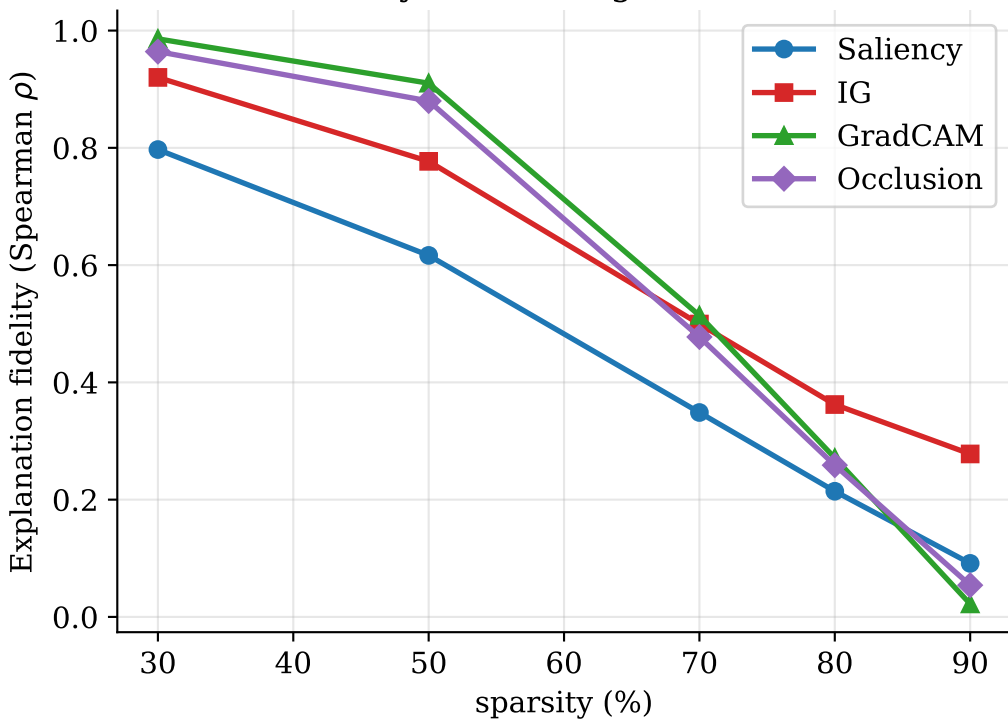
Fidelity vs. Pruning (CIFAR-10)
