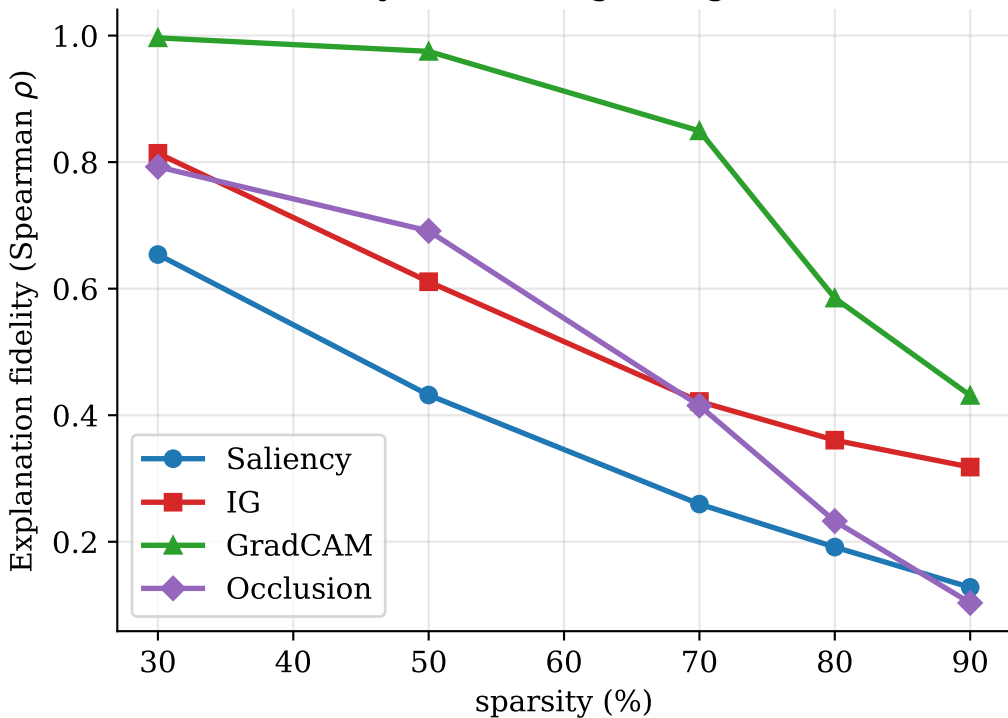
Fidelity vs. Pruning (ImageNette)
