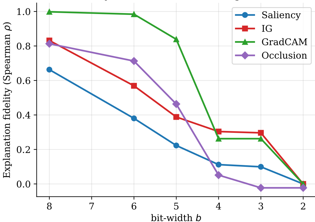
Fidelity vs. Quantization (ImageNette)
