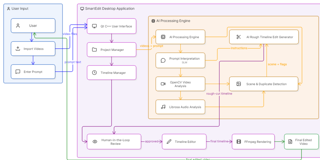
Fig. 5.1: System Architecture of the SmartEdit AI-Assisted Video Editing System.
