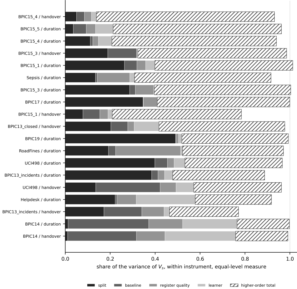
Figure 2: First-order sensitivity indices per log–target pair, within instrument, under the equal-level measure. Each segment is the median over the five instruments of that axis’s index, and the hatched segment is the median of the total higher-order share 1 - \sum_i S_i of (3). The bars therefore need not sum to one, and a few exceed it: medians do not add. The dotted rule marks one. The figure carries no intervals; the bootstrapped indices and their intervals are in Table 3.
