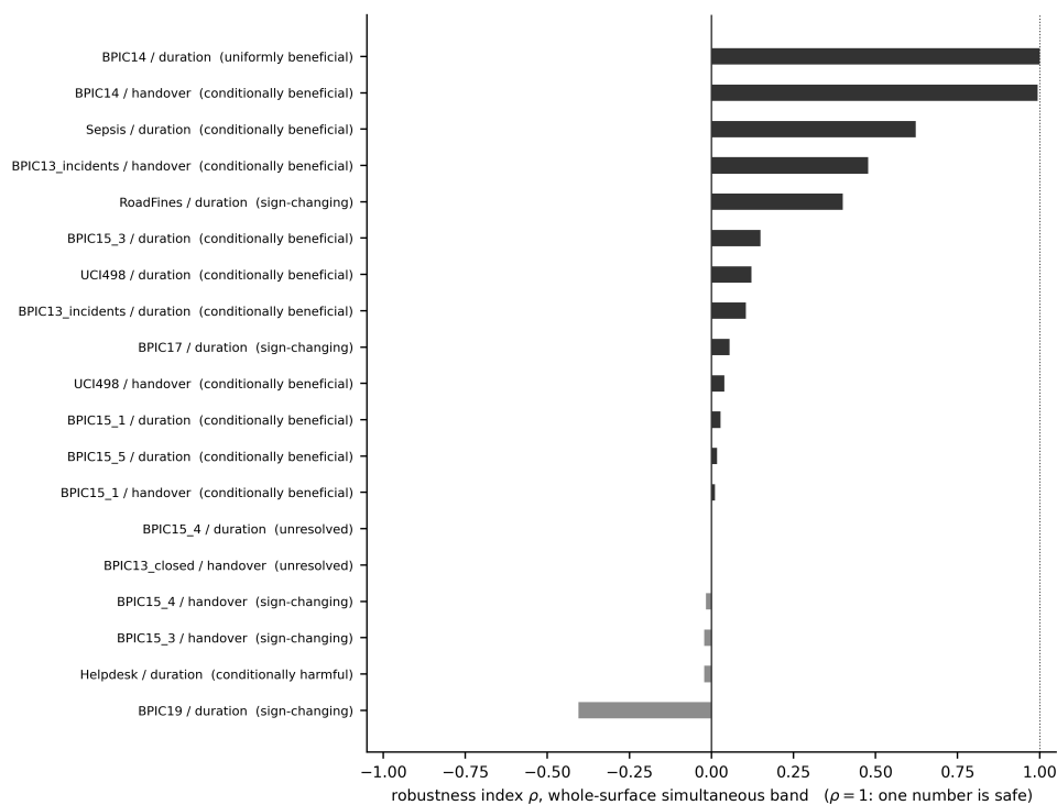
Figure S4: The robustness index \rho per log–target pair, with the region label, at the critical value Section 6.3 reports. \rho = 1 , the dotted line, is the only state in which a single positive number is a safe summary.
