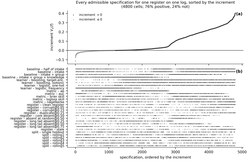
Figure 1: The specification curve for the configuration item on BPIC14, at the registered handover target: 4,800 admissible scalar cells, 4 pipelines \times 4 baseline runs \times 5 instruments \times 10 register-quality conditions \times 6 splits. (a) Each point is one admissible specification — a complete assignment to those five axes — sorted by the increment. (b) Which level of which axis each specification occupies. The intercept-only rung is excluded. Every point is a point estimate; the simultaneous bands that decide the region labels are in Table S9. The five scalar instruments are plotted on one axis and their increments are not on a common scale (Section 4.7); what the panel supports is the sign statement, which is unit-free, and not a comparison of magnitudes across instruments. The panel shows the increment rather than the reduction, so a cell where the register is worth almost nothing looks the same as one where the free field absorbs almost everything.
