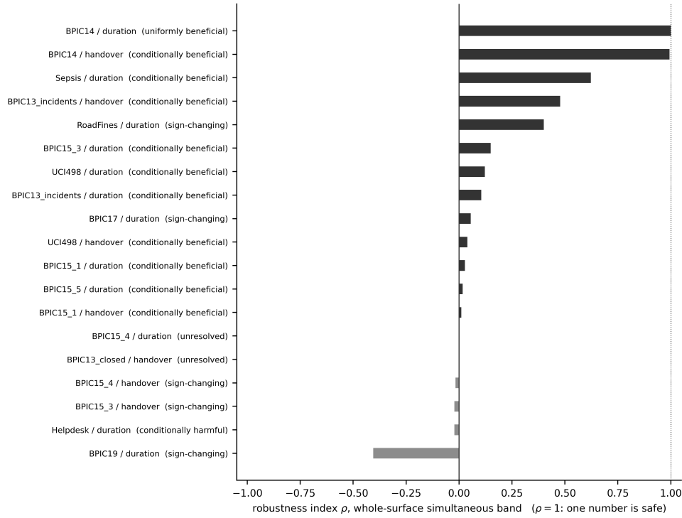
Figure S4: The robustness index \rho per log–target pair, with the region label, at the critical value Section 6.3 reports. \rho = 1 , the dotted line, is the only state in which a single positive number is a safe summary.
