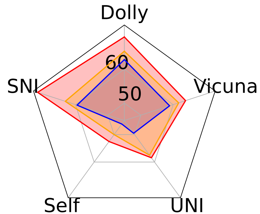
7B -> 0.5B
