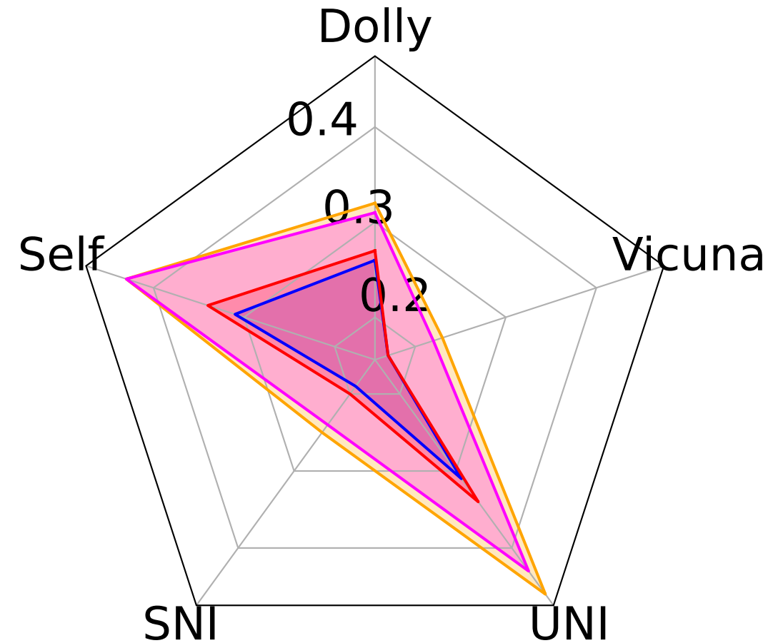
Qwen2.5-1.5B
