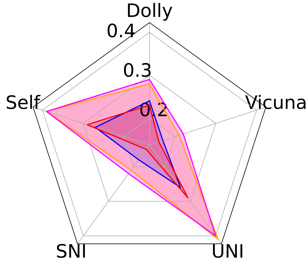
Qwen2.5-0.5B
