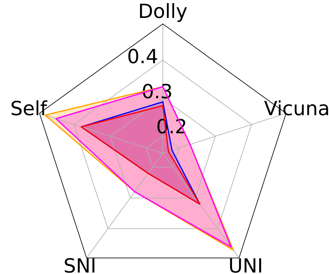
Qwen2.5-7B
