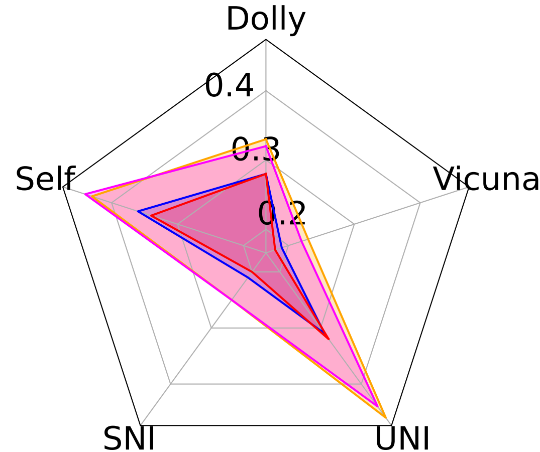
Qwen2.5-3B
