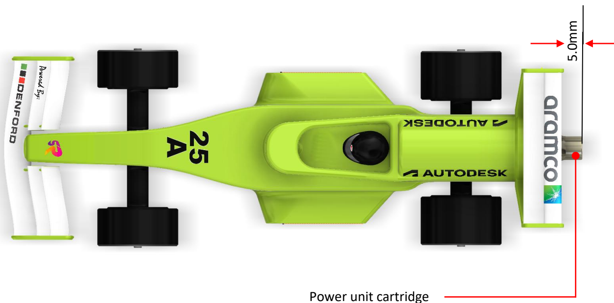
T5.6: Minimum protrusion in top, bottom and side view
