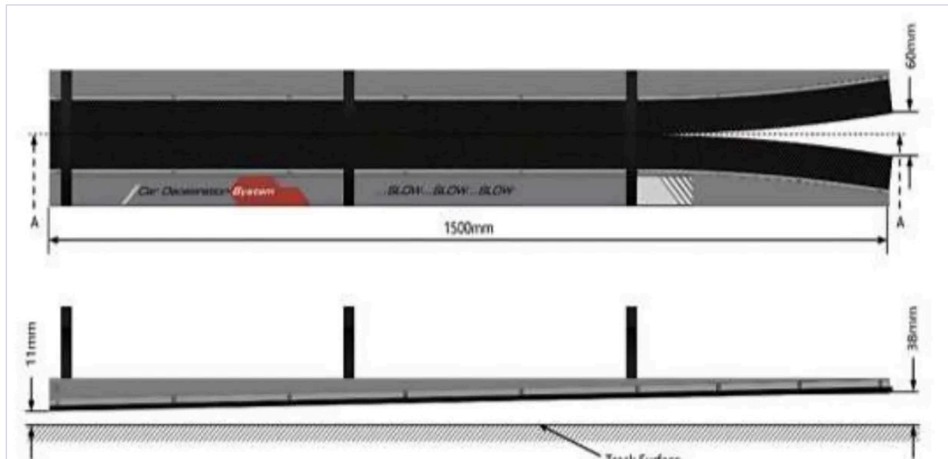
The car deceleration system after the finish line (Appendix vii).
