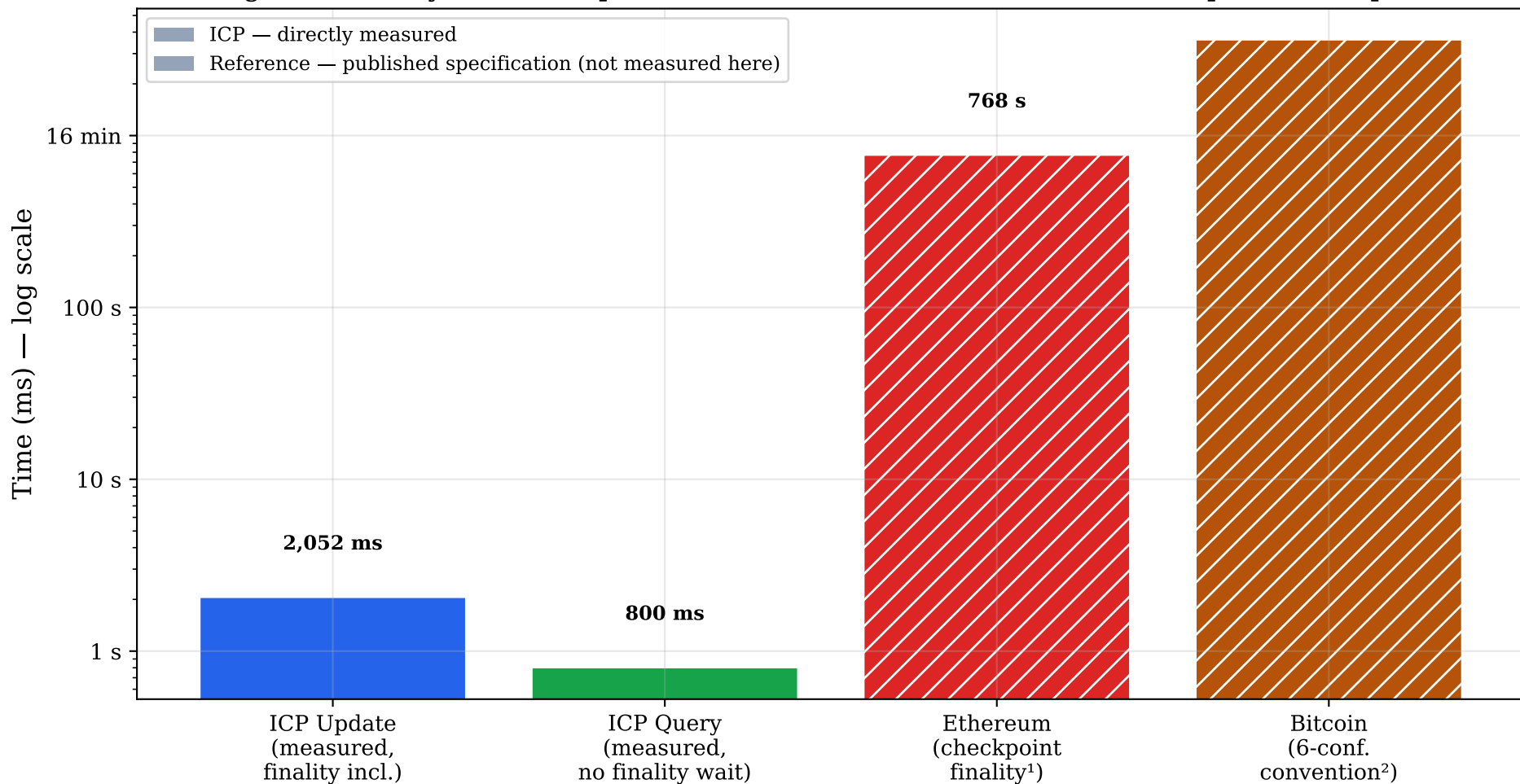
Fig 7 — Finality Time Comparison: ICP (measured) vs Other Chains (published specs)
