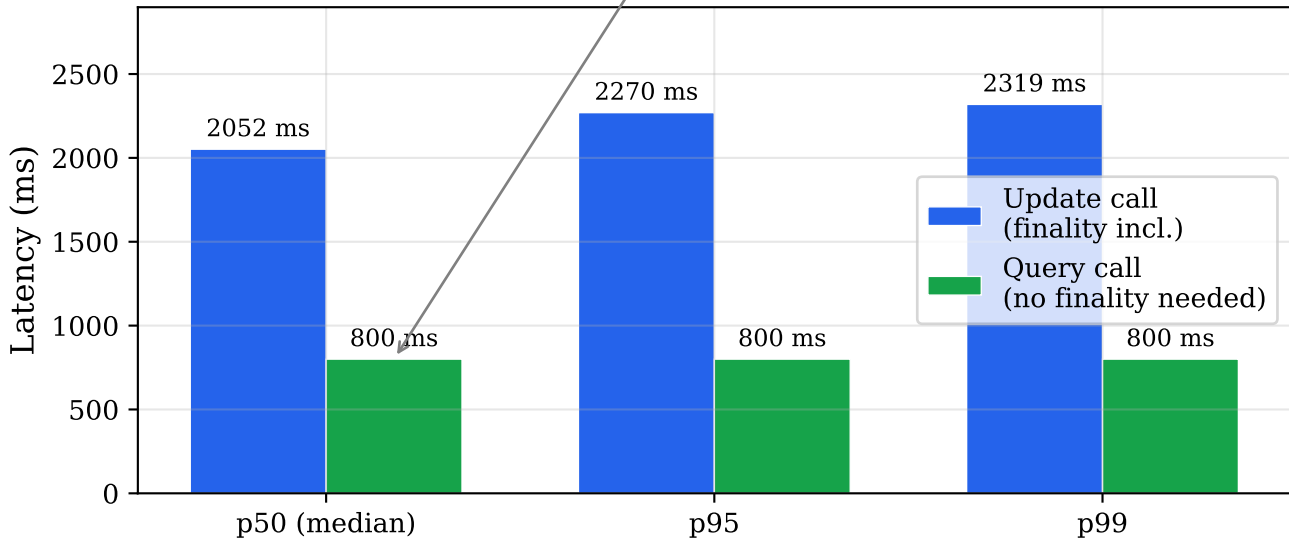
Fig 1 — ICP Update Call vs Query Call Latency (Update call = finality included; Query call = instant read)
