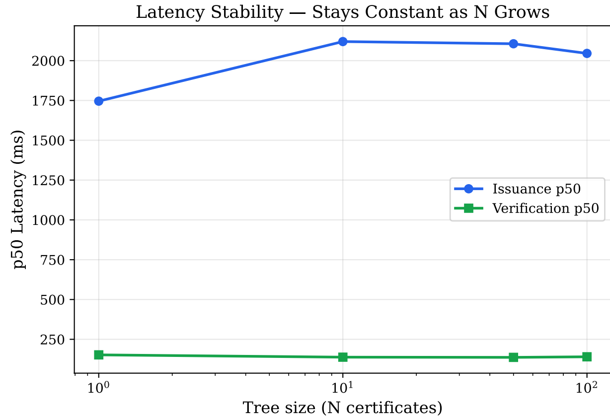
Fig 8 — ICP Scalability Claims: Throughput & Latency Stability
