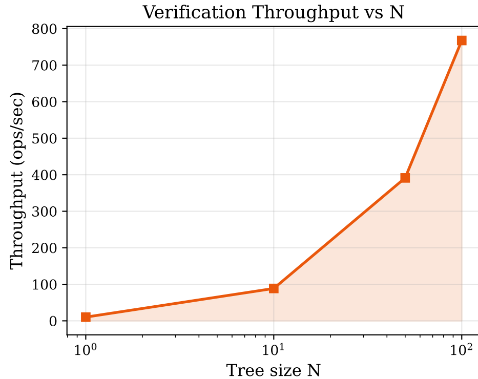
Fig 3 — Verification Scalability (O(log N) Merkle Proofs)
