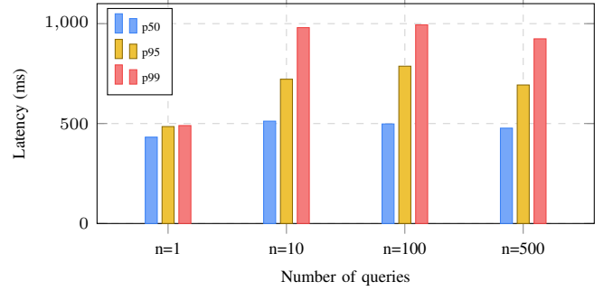
Fig. 4. Verification latency (p50/p95/p99) for different batch sizes. Each batch of n queries is issued sequentially. p99 stays below 1 second across all scales.
