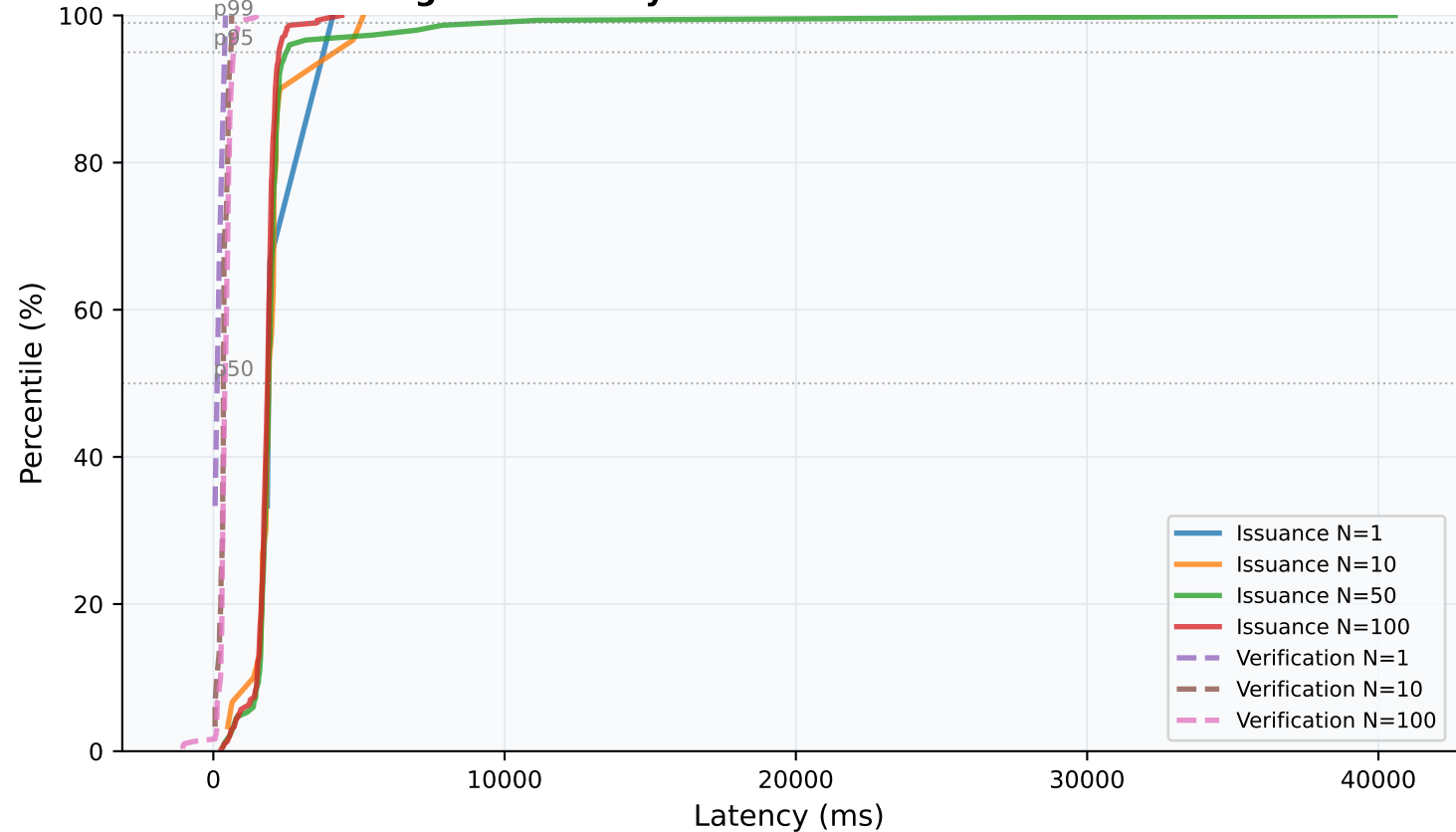
Fig 5 — Latency CDF: Issuance vs Verification
