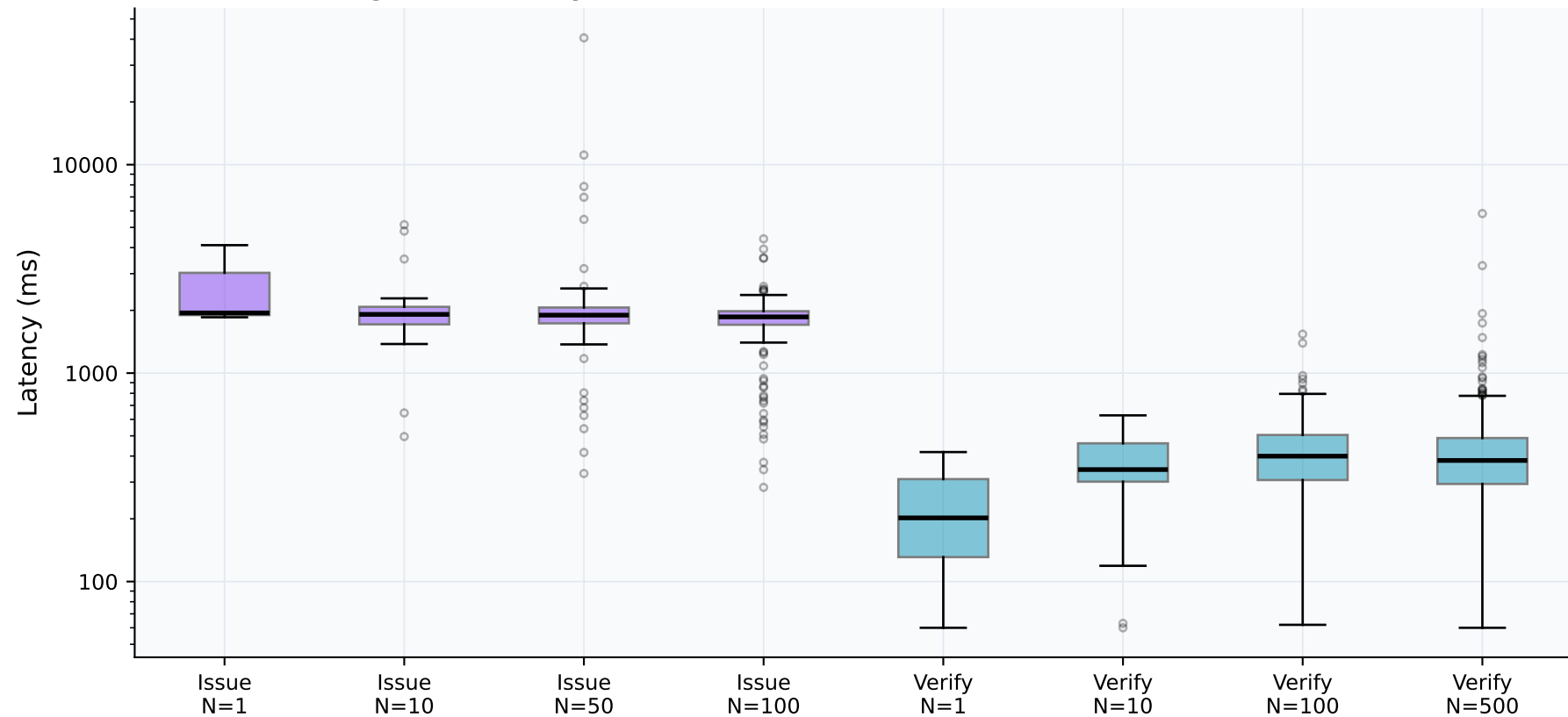
Fig 7 — Latency Distribution: Issuance vs Verification (Box Plots)
