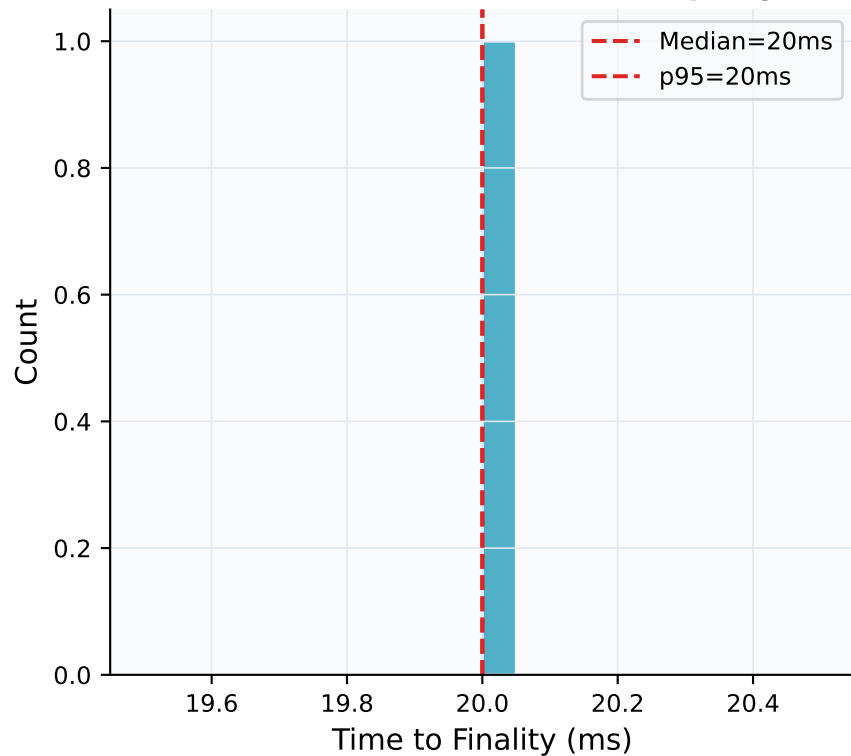
Fig 10 — ICP Consensus Finality Time ICP Finality Time Distribution (submit → cert readable via query)
