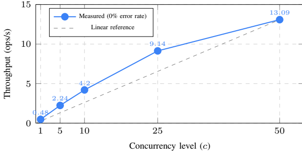
Fig. 6. Mixed-workload throughput (30% issue, 70% verify). Sub-linear growth is because issuance calls are serialized per consensus round.
