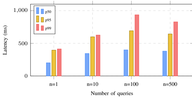
Fig. 4. Verification latency (p50/p95/p99) for different batch sizes. Each batch of n queries is issued sequentially. p99 stays below 1 second across all scales.
