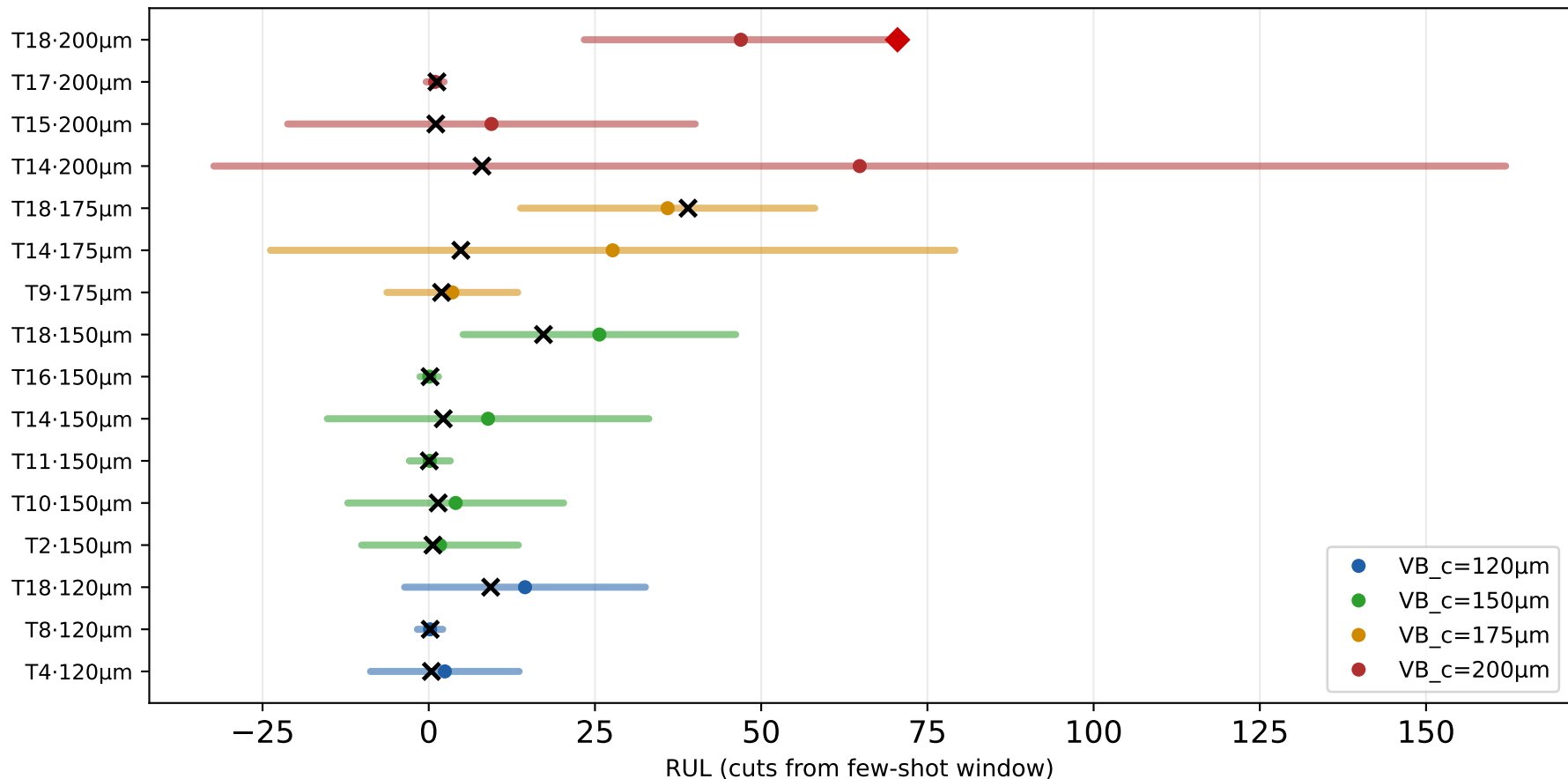
Calibrated RUL windows: 94% of 16 events contain the truth (bar = 90% window · o = predicted · × = covered · ◇ = missed)
