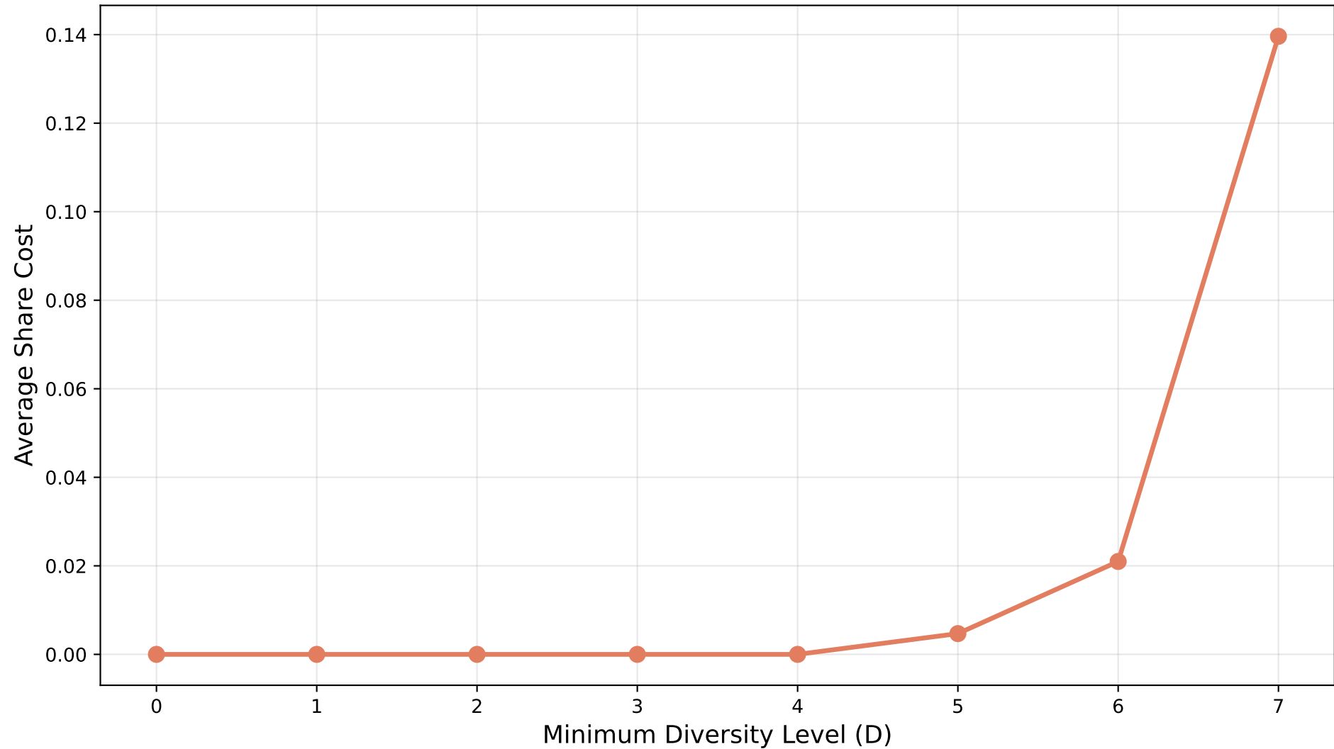
Marginal Cost of Increasing Diversity
