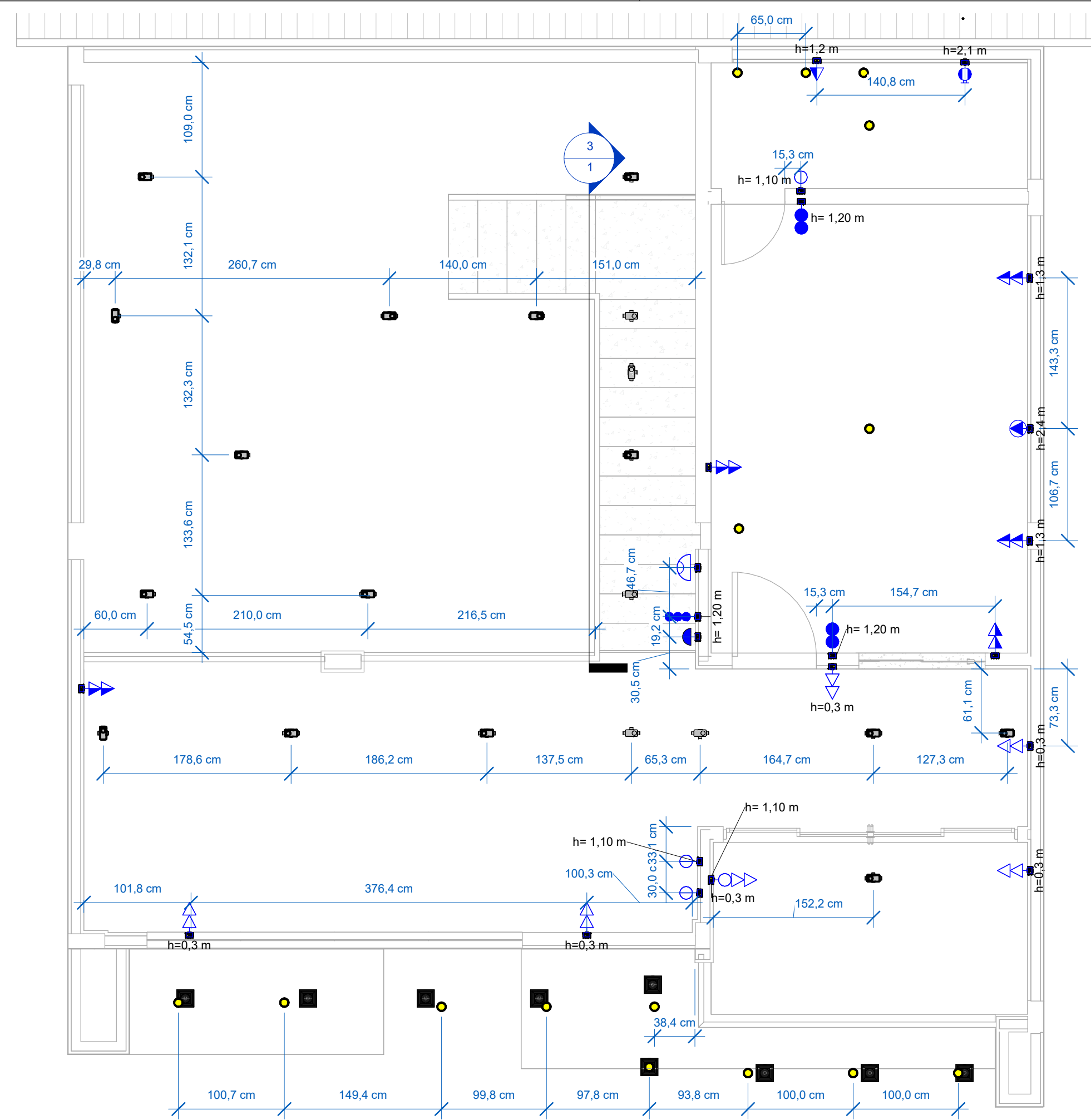
2 SUPERIOR-ELT LAYOUT 1 : 40
