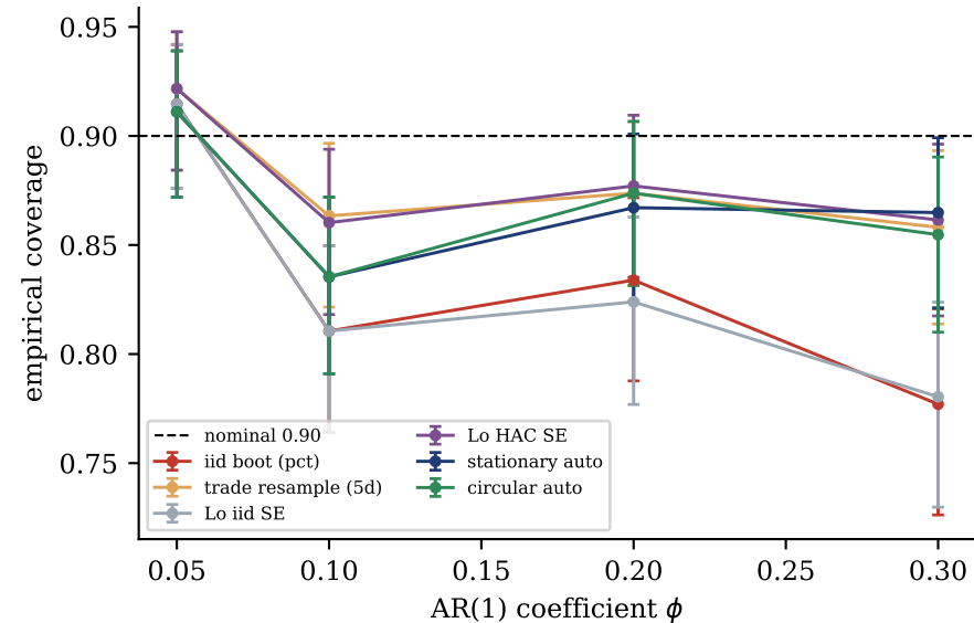
(a) AR(1): coverage vs \phi (pooled over T )
