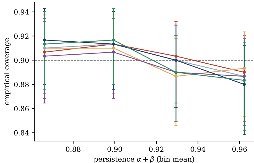
(b) GARCH(1,1): coverage vs persistence \alpha + \beta
