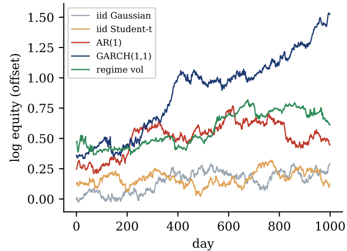
(a) cumulative log-equity (offset), true SR = 1
