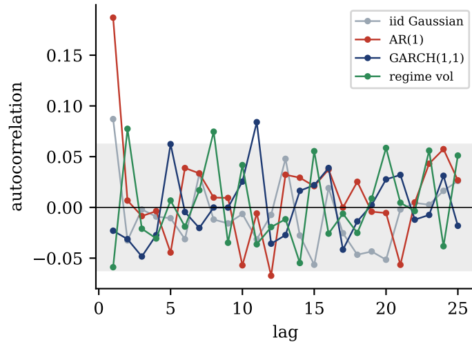
(b) ACF of returns
