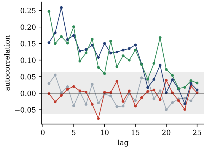
(c) ACF of squared returns (vol clustering)
