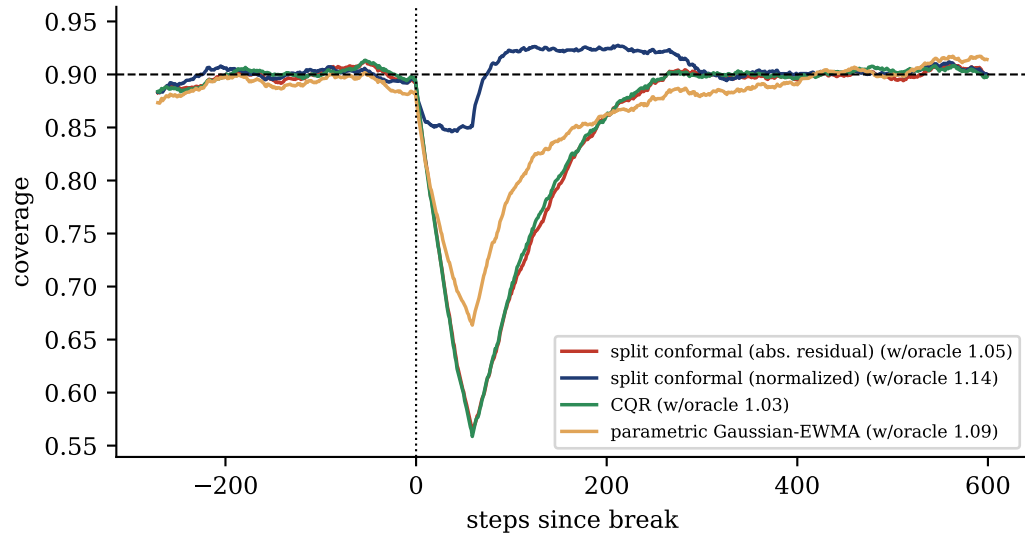
(a) coverage around the break (rolling 60 steps)
