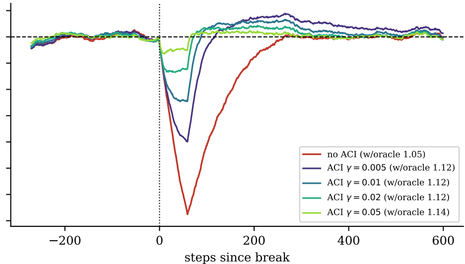
(b) ACI repair speed vs \gamma (abs. score)
