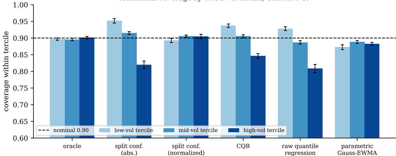
conditional coverage by TRUE-vol tercile, GARCH DGP
