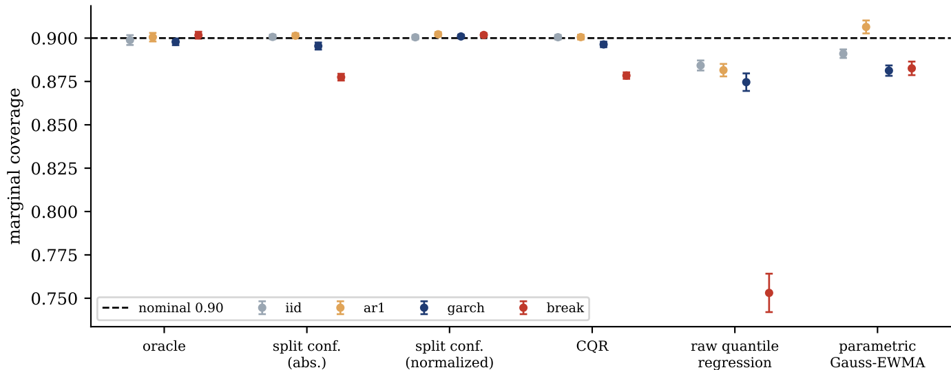
marginal coverage by method and DGP (95% CIs over experiments)
