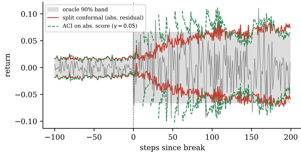
(b) abrupt vol break ( \times 4 ): the coverage hole
