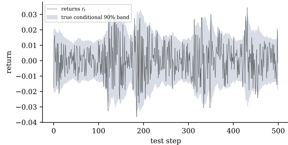
(a) GARCH(1,1) DGP: the truth is known
