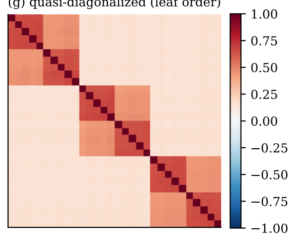
(g) quasi-diagonalized (leaf order)
