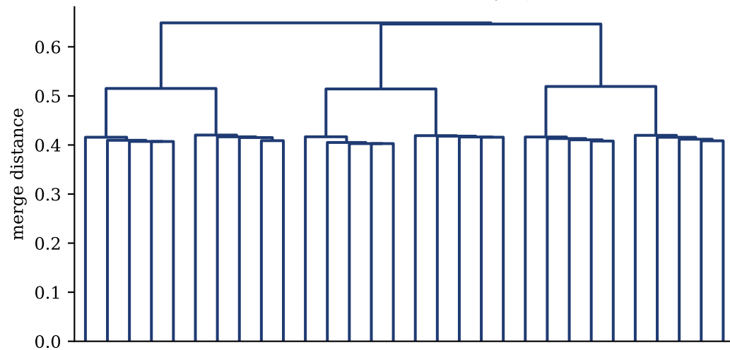
(e) single-linkage dendrogram on d_{ij} = \sqrt{(1 - \rho_{ij})/2}
