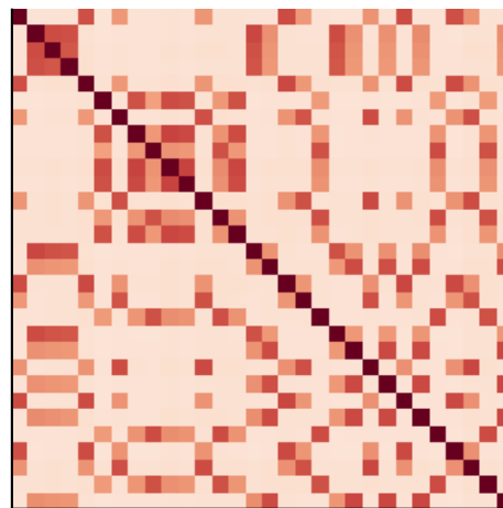
(f) hierarchical, shuffled order
