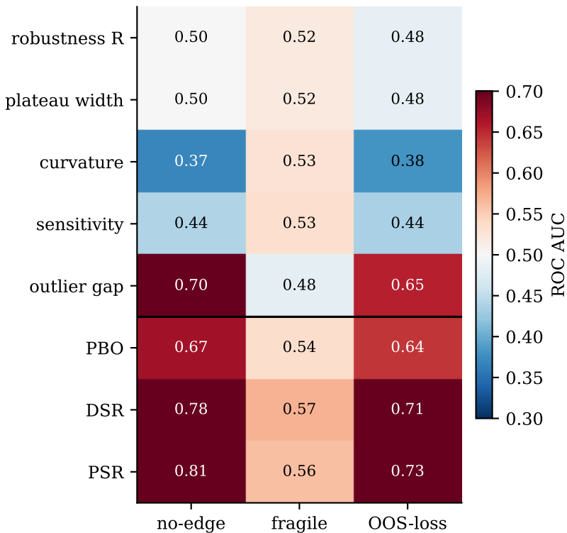
Overfitting-mode detection (AUC)
