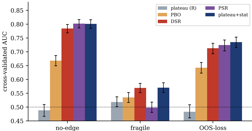
Single diagnostics vs. a combined geometry+statistics classifier
